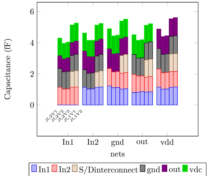
Fig. 8: For each net configurations of a NAND cell 1 to 5 are shown in parallel. The three first configurations are 2stacked gates technology (JL2V1, JL2V2, JL2V3) while the last configurations are single gate technology (JL1V1, JL1V2). For the two JL1 configurations, an additional interconnect capacitance (S/D interconnect) is measured.
