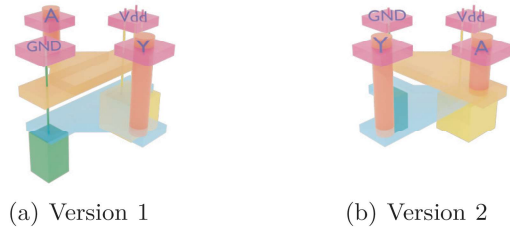
Fig. 6: 3D representation of a CMOS inverter using the octilinear routing style and our VNWFET technology
