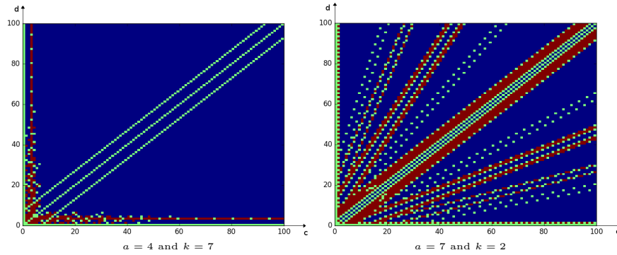
Figure 1: Properties of the outcome sequences for G = (\{a, a + k\}, \{c, d\}) . The parameters a and k are fixed, and the pictures are obtained by varying the parameters c and d . The point at coordinate (c, d) is blue if the corresponding game is eventually \mathcal{L} , red if it is eventually \mathcal{R} , and green if there is a mixed period.
