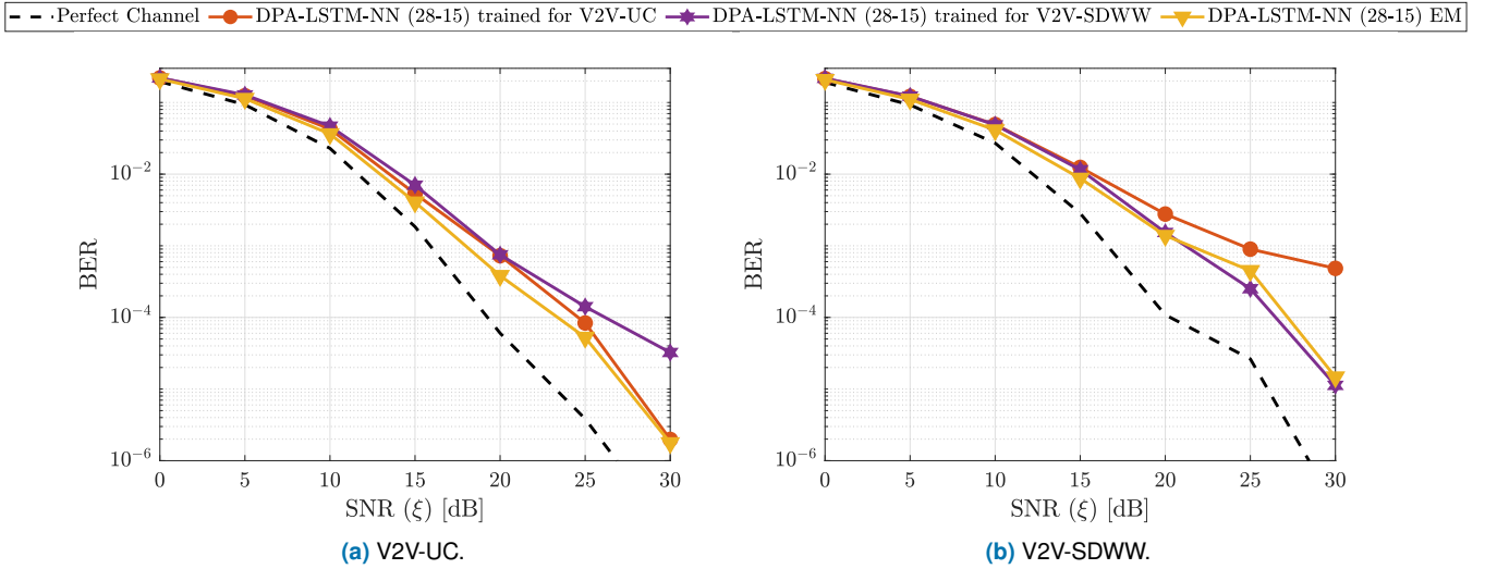
FIGURE 17: BER performance of the proposed DPA-LSTM-NN scheme with QPSK modulation, v = 100 km/h and IBO = 2 dB, using Ensemble Modeling.
