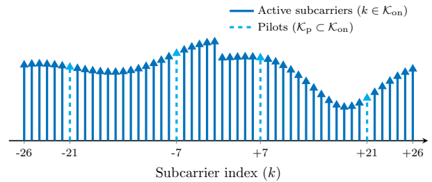
(a) Active subcarriers, including pilots.
