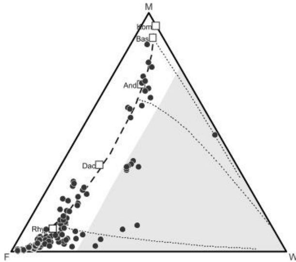
Fig. 3. FMW ternary diagram after Ohta and Arai (2007) for the whole-rock geochemistry database. Samples that plot on the shaded area indicate higher degree of weathering and were not considered for the results and discussion sections.
