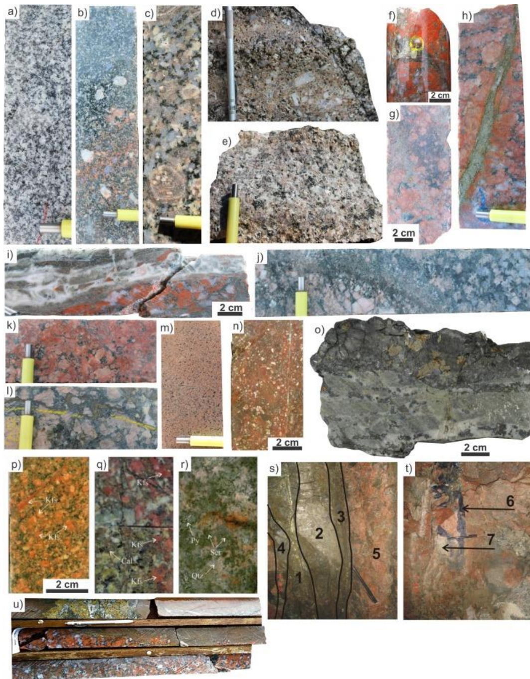
Fig. 2. Typology of the different OMS (a – o) and YMS rocks (p – u). (a) Massive, leucocratic, granodiorite drill core sample. (b) Massive, partially altered (potassic alteration), granodioritic porphyry; (c) Porphyritic and massive syenogranite with compositionally zoned plagioclase phenocrysts; (d) Syenogranitic porphyry with plagioclase phenocrysts (outcrop near the Patrocínio area); (e) Equigranular, massive monzogranite; (f) Strongly altered (potassic alteration) granite, with gold bearing pyrite in chlorite-sericite veinlets; (g) Sulfide bearing, chlorite-sericite alteration in K-metasomatized granitoid; (h) Gold bearing, quartz sulfide vein injected near the granite-syenite contact. Rocks have previously experienced pervasive potassic and subsequent chlorite-sericite alteration; (i) Granite drill-core sample with multi-phasic hydrothermal events. early potassic alteration (reddish feldspar crystals) is followed by fissural and interstitial chlorite-sericite alteration (gray-greenish color). The last hydrothermal event is represented by the white-silica infilled breccia; (j) Drill core sample with contact between monzonite (left) and monzogranite (right) with a reaction rim (central) and small opaque (sulfide?) crystals; (k) Potassic and chlorite-sericite altered syenite; (l) Chlorite-sericite and potassic altered monzonite with disseminated, gold bearing sulfide (pyrite and pyrrhotite), and less frequent sulfide veinlets; (m) Aplitic syenite found as synplutonic dykes in OMS granites. (n) Rhyolite with feldspar phenocrysts and potassic alteration from the Coringa deposit; (o) Coringa deposit ore example, with strongly sericitic altered volcanic rock (rhyolite?) cross-cut by a chalcopryite + sphalerite + galena vein, brecciated by sericitic + white silica alteration. (p – t) Palito deposit samples (examples from Echeverri-Misas, 2015; (p) potassic altered granite with secondary K-feldspar; (q) potassic and propylitic alteration with K-feldspar, chlorite, epidote and carbonate (Cal); (r) Sericitic alteration with quartz (Qtz), sericite (Ser) and pyrite (Py); (s) Sulfide vein in strongly hydrothermalized granite (5), with (1) chalcopryite, (2) pyrite, (3) breccia zone and (4) quartz veins; (t) Strongly hydrothermalized granite with fluorite (6) and white silica veining (7). (u) OMS granite injected by YMS dacite dyke with white silica, gold bearing sulfide pocket and smaller veinlets along the dyke contact.
