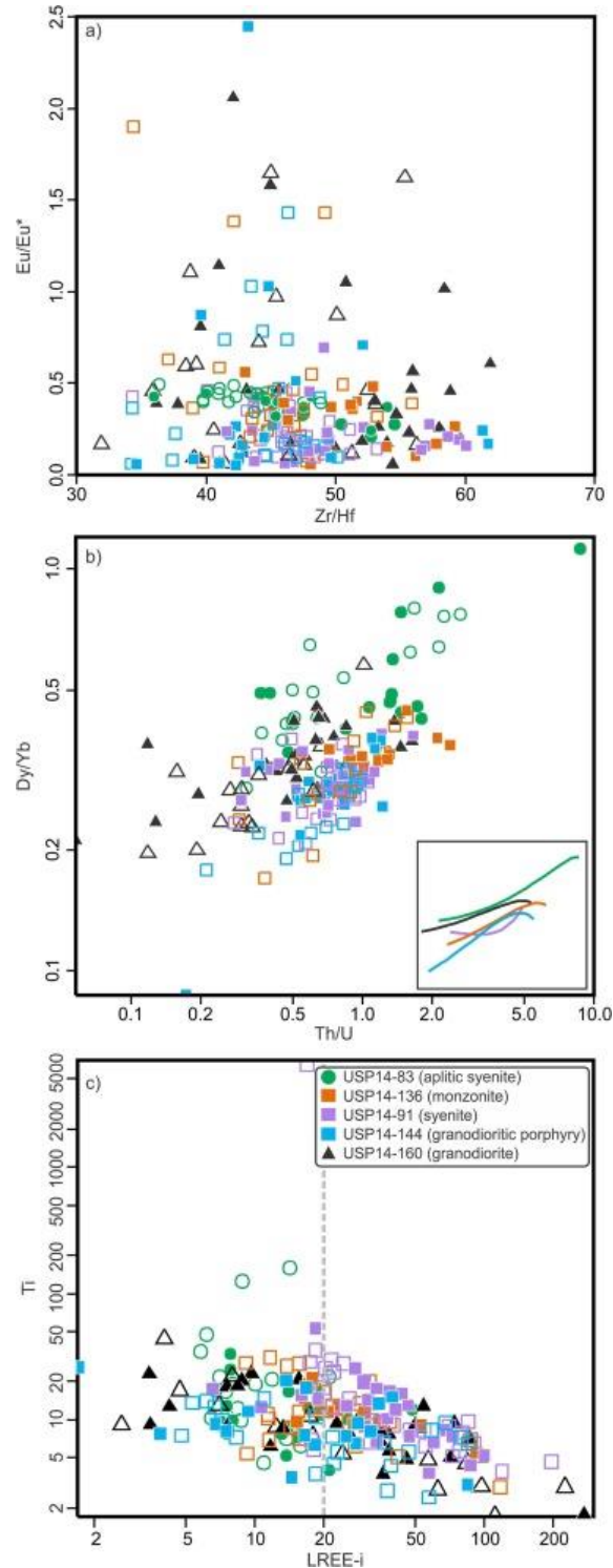
Fig. 11. Zircon geochemistry with \text{Zr}/\text{Hf} vs. \text{Eu}/\text{Eu}^* (a) and \text{Th}/\text{U} vs. \text{Dy}/\text{Yb} plots (b), where both \text{Zr}/\text{Hf} and \text{Th}/\text{U} ratios were used as proxies for differentiation. Bottom right smaller graph in (b) shows the polynomial regressions with the general trend for each sample. (c) Light REE index (LREE-i) as proposed by Bell et al. (2016) vs. Ti plot. The index is calculated as \text{LREE-i} = (\text{Dy}/\text{Nd} + \text{Dy}/\text{Sm}) , in order to constrain the proportion between middle and light-REE in zircon grains. Grains with low LREE-i show high LREE content, which might indicate hydrothermal alteration (or LREE rich inclusions such as apatite or monazite on the ablated spot).
