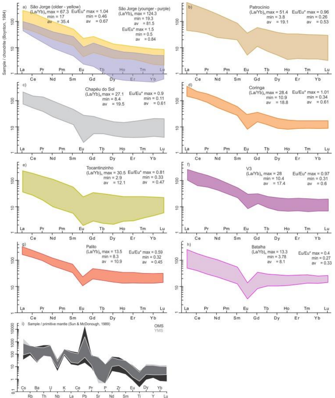
Fig. 8. Chondrite normalized (Boynton, 1984) REE spidergrams for the OMS (a – e), YMS (f – h) and trace-element spidergrams normalized by the primitive mantle (Sun and McDonough, 1989) for both sequences. The respective colored fields represent the entire range covered by each deposit/unit. Eu anomaly calculated as Eu/Eu^* = Eu/N
