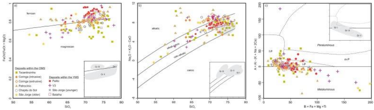
Fig. 5. Frost's classification diagrams for OMS and YMS, with SiO 2 vs. Fe-index (a), SiO 2 vs. MALI (b), and A-B diagram after Villaseca et al. (1998) (c), where A = Al - (K + Na + 2Ca) and B = Fe + Mg + Ti , calculated for milcations. Extrusive rocks from the Coringa and V3 deposits are plotted for comparison purposes.
