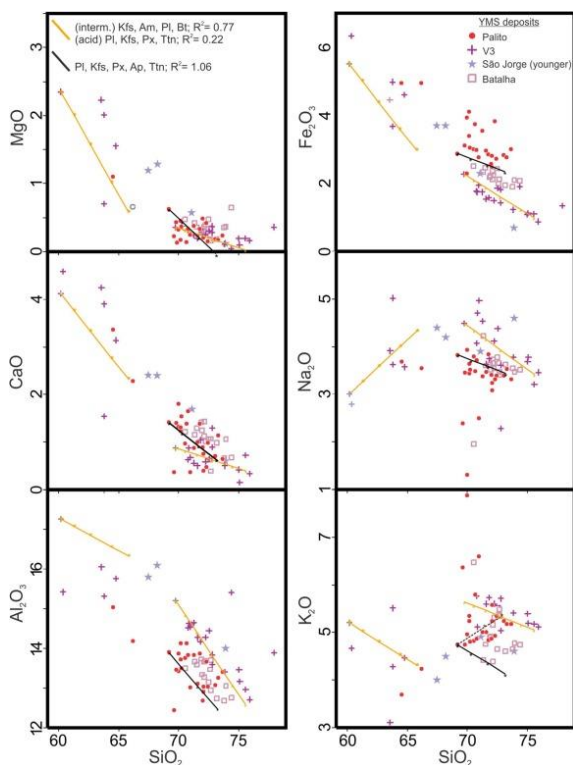
Fig. 7. Silica vs. major oxides for YMS rocks. Yellow and black arrays mark the petrologic trends modeled, with the minerals involved and the R2 parameter indicated at the top. Symbols are the same as in the previous figures. Abbreviations: Kfs (K-feldspar), Am (amphibole), Pl (plagioclase), Bt (biotite), Px (pyroxene), Ttn (titanite), Ap (apatite).
