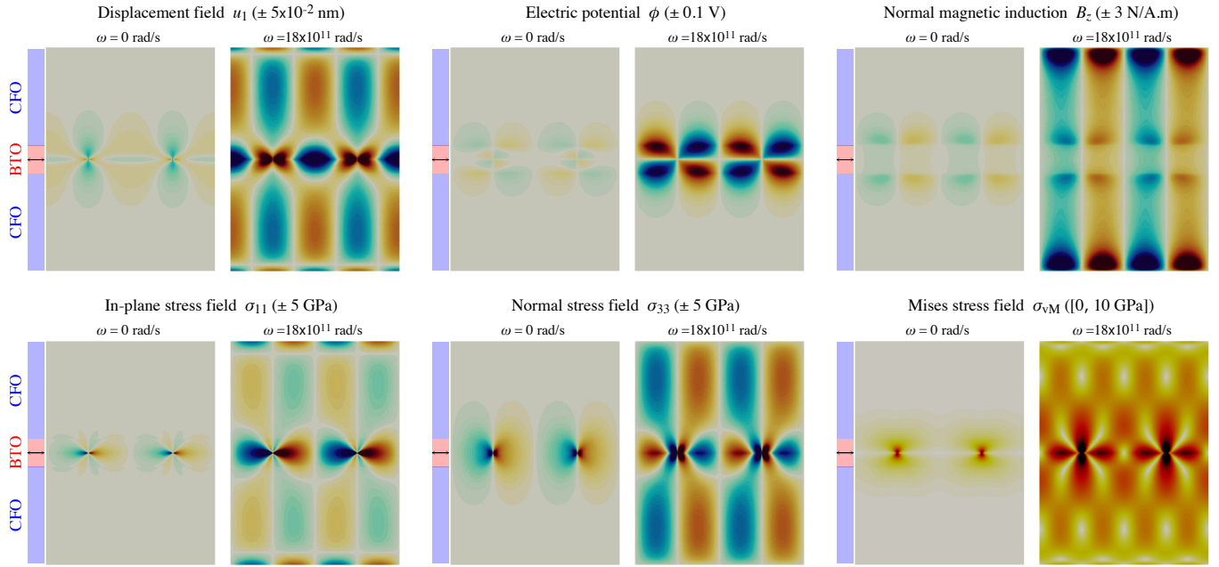
Figure 10: Effect of the frequencies on the nonlocal MEE field solutions induced by a time-harmonic tilt grain boundary of edge dislocations in a free-standing a CFO/BTO/CFO trilayered system. The blue (red) color with negative (positive) values represents the minimum (maximum) magnitude of the corresponding field components, while zeros are shown in white.
