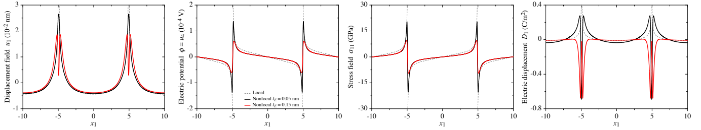
Figure 7: Influence of the nonlocal parameter on the static MEE field components produced by a tilt grain boundary in a homogeneous BTO material. The boundary is described by an infinitely long, straight and uniformly spaced parallel dislocations with edge characters. Curves are plotted along the tilt boundary for two nonlocal parameter values, while the local MEE calculations are shown for comparison.
