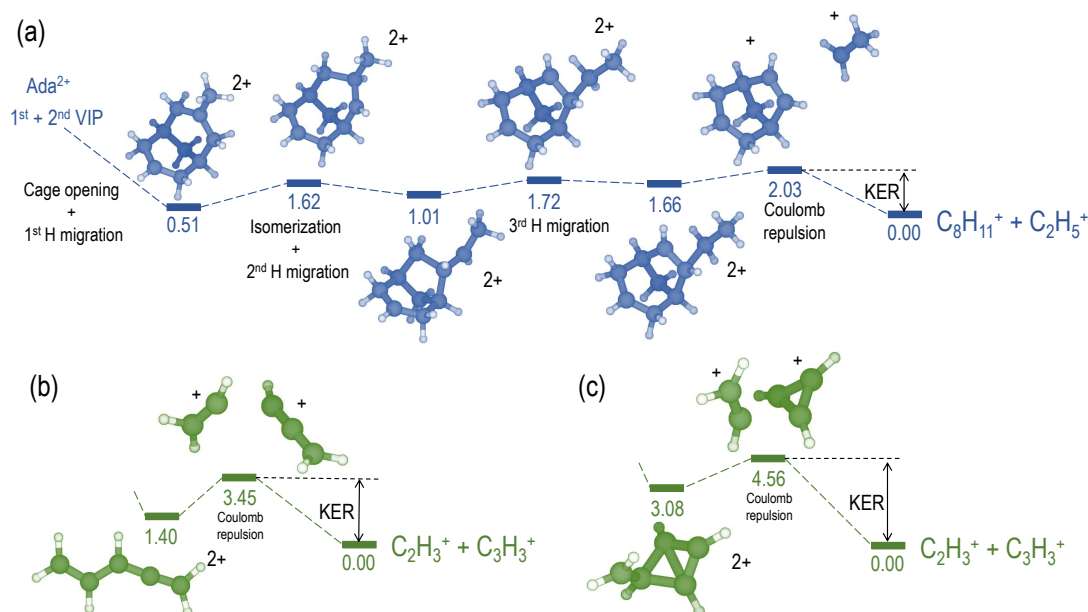
Fig. 8 Potential energy surfaces (DFT-B3LYP/6-31G(d) level) for the channels \text{C}_2\text{H}_5^+/\text{C}_8\text{H}_{11}^+ (a) and \text{C}_2\text{H}_3^+/\text{C}_3\text{H}_3^+ (b-c). Relative energies in eV corrected with ZPE and referred to the corresponding exit channel.
