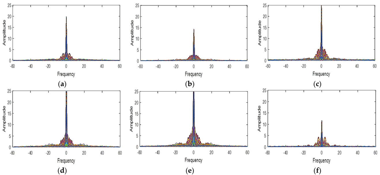
Figure 6. The power spectrum functions of the gradient signal in beers image (a) green–red (b) green–blue (c) green–orange (d) red–blue (e) red–orange (f) blue–orange.
