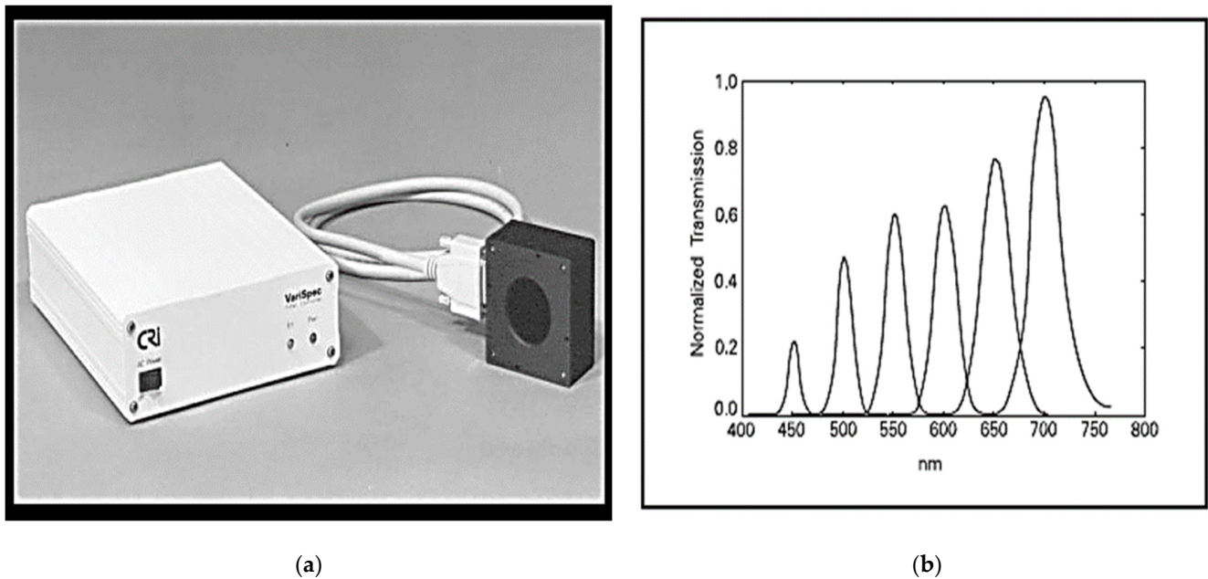
Figure 2. (a) The LCTF (b) The LCTF at several wavelength settings [19].
