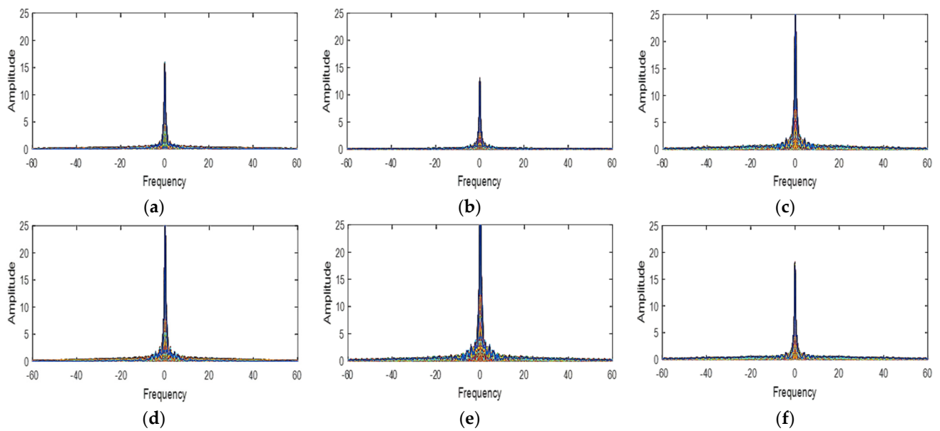
Figure 5. The power spectrum functions of the gradient signal in hairs image (a) green–red (b) green–blue (c) green–orange (d) red–blue (e) red–orange (f) blue–orange.
