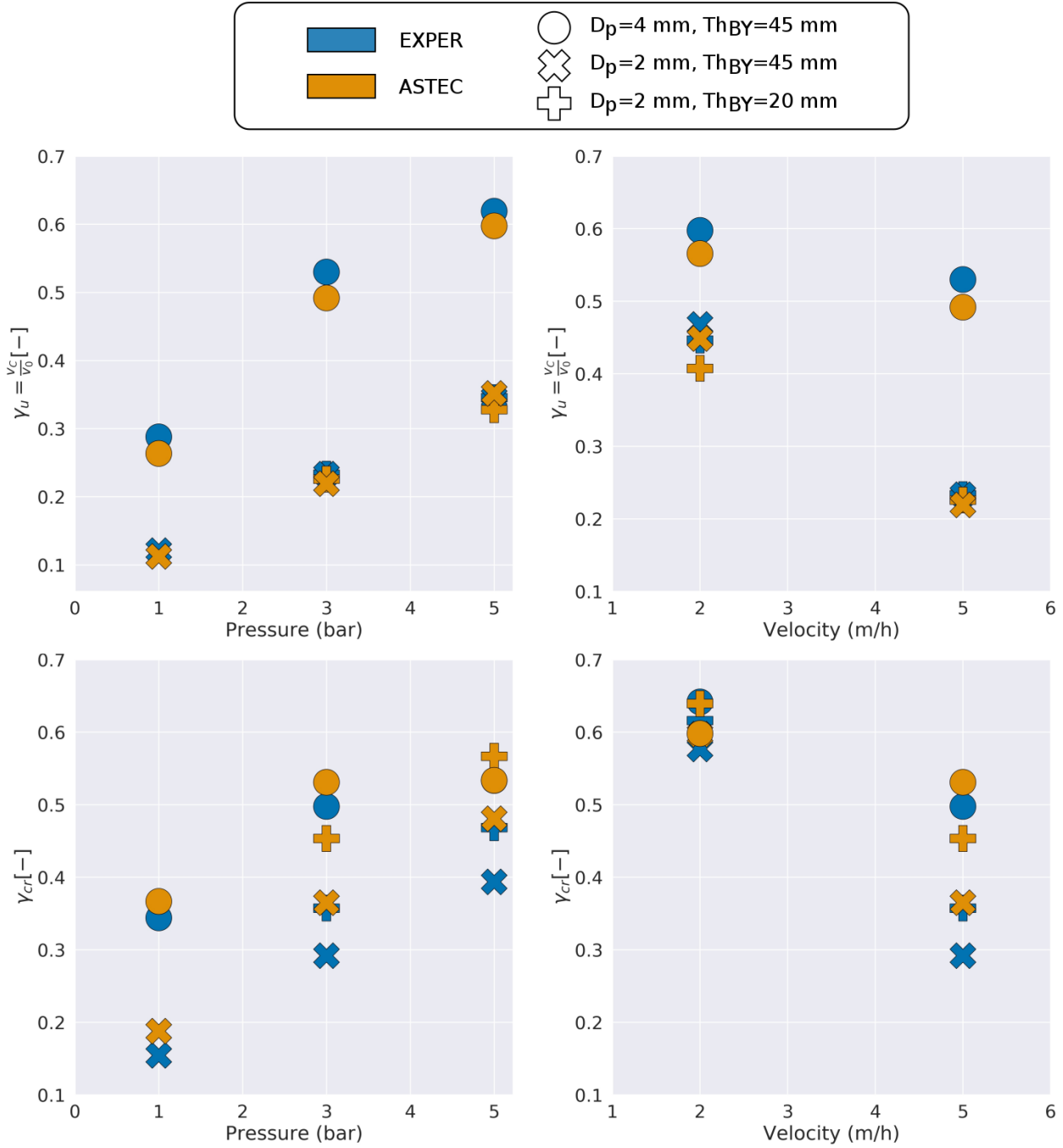
Figure 10: Experimental and Predicted quench front velocity ratio ( \gamma_u ) and conversion ratio ( \gamma_{cr} ) as a function of the system pressure (injection velocity of 5 m/h) and the injection velocity (system pressure of 3 bar) for different bed configurations. Initial debris temperature of 700 °C in all cases.
