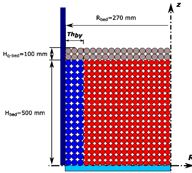
Figure 3: Axial view of the PEARL debris bed with ASTEC V2.1: red beads represent the heated central bed (C), blue beads represent the bypass (BY) and grey beads represent upper quartz bed (Q). The bottom of the central bed and bypass are located at z = 0 mm.
