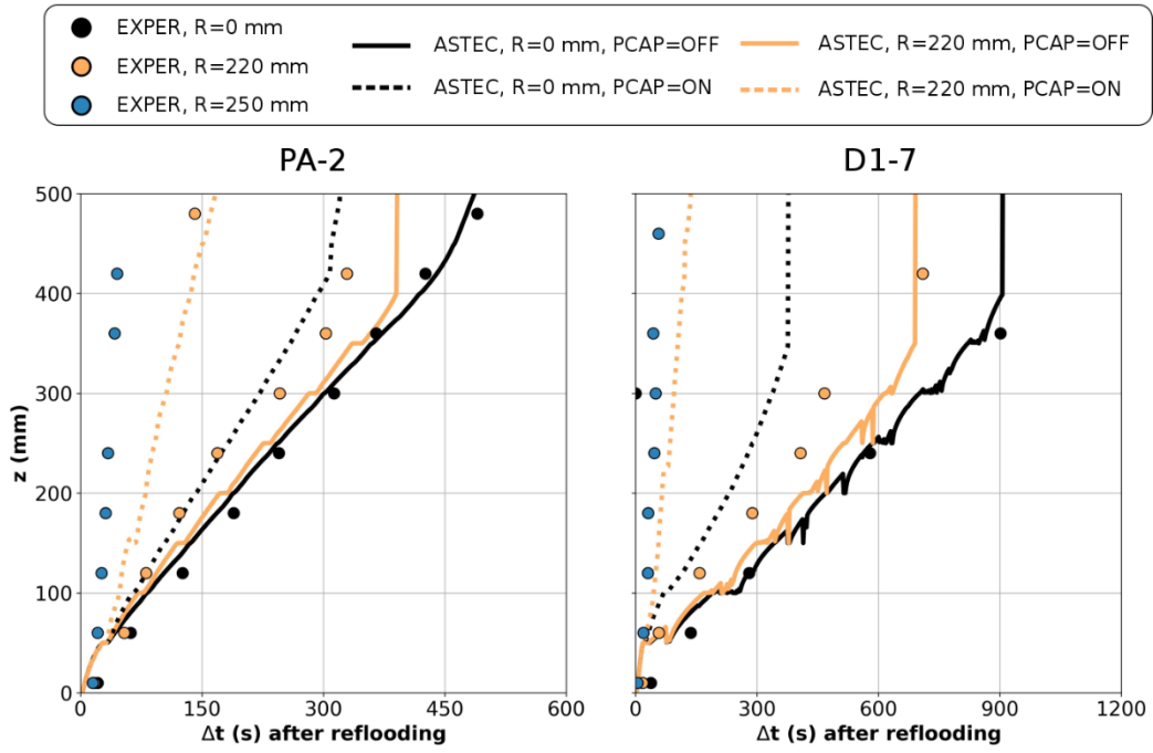
Figure 11: Predicted vs. Experimental evolution of the quench front for the tests PA-2 and D1-7 (see Table 1) with and without the capillarity correction.
