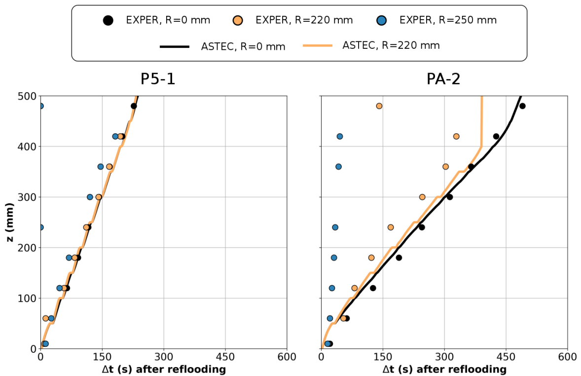
Figure 4: Predicted vs. Experimental quench front evolution for the tests P5-1 and PA-2.
