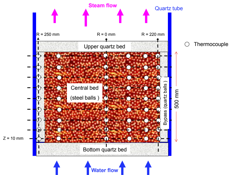
Figure 2: Debris bed structure and instrumentation. The radial positions of the instrumented vertical axis correspond to the values for the beds 1 and 2-1.
