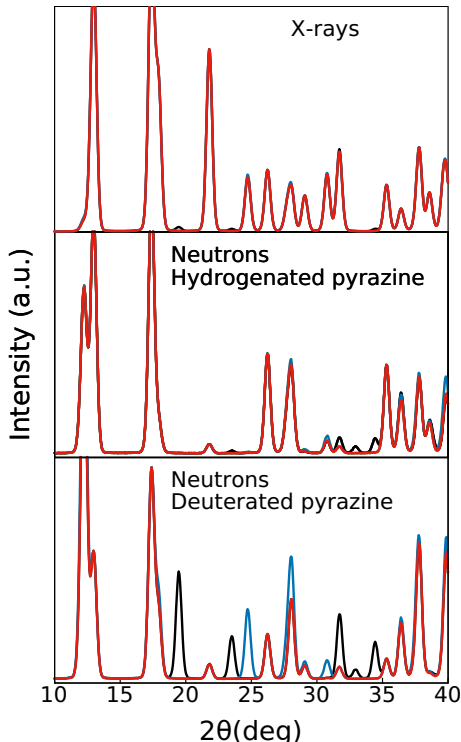
Figure 2. Simulated powder diffraction patterns (wavelength 1.54 Å) of Fe(pyrazine)[Pt(CN) 4 ] in low-spin state with the pyrazine rings in disordered configuration (red lines), in ordered perpendicular (black lines) and parallel (blue lines) configurations: (top) X-rays and hydrogenated pyrazine; (middle) neutrons and hydrogenated pyrazine; (bottom) neutrons and deuterated pyrazine.
