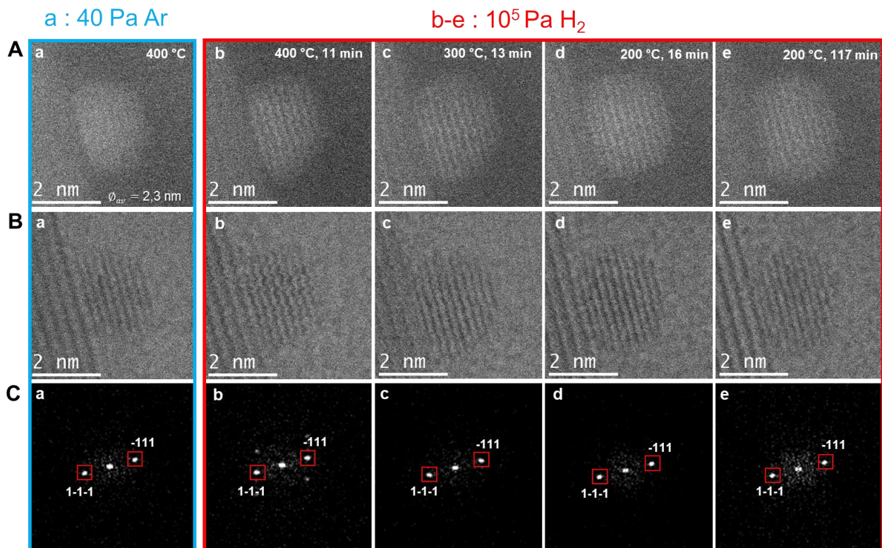
Figure 2: Atomic scale visualization of the structural stability of a Au-Cu NP of a size of 2.3 nm supported on anatase TiO_2 support in H_2 at atmospheric pressure. (A-B) STEM HAADF (A a-e)
