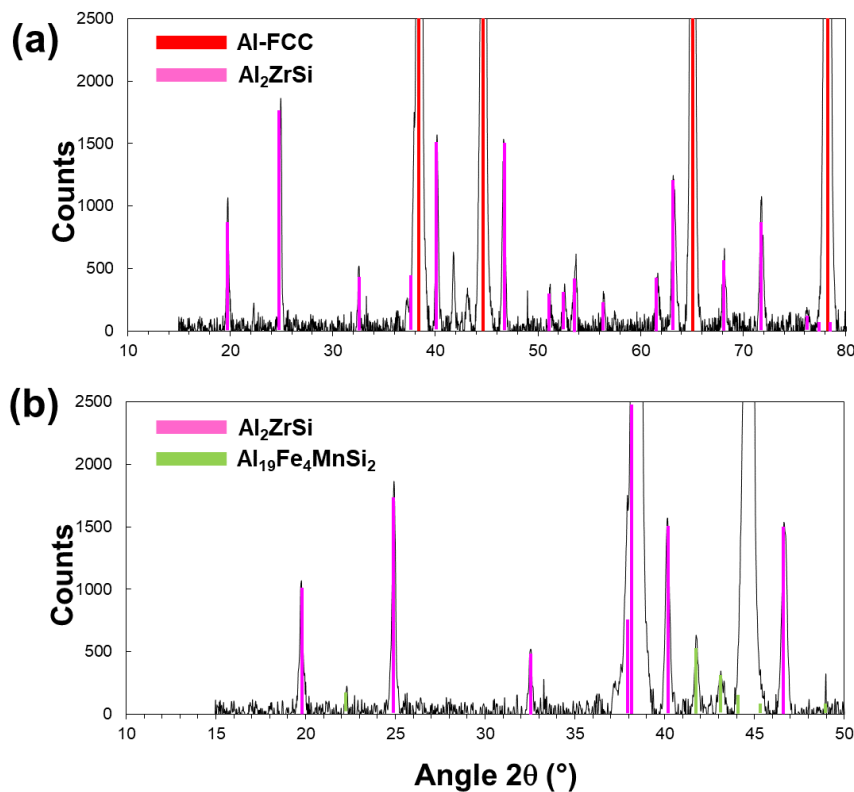
Figure 7. XRD pattern collected on a sample subjected to 550°C/30min. (a) in the (10°, 80°) angular range, the main diffraction peaks are indexed as FCC-Aluminium ( a = 4.05 \text{ \AA} , red lines) and tetragonal \text{Al}_2\text{ZrSi} phase (Pearson symbol tI8 14/mmm (139) , a = b = 3.88 \text{ \AA} , and c = 8.98 \text{ \AA} , pink lines). (b) Enlarged views of the XRD patterns in the 10-50° range. The green lines can be indexed as a cubic structure with a large lattice parameter a = 12.60 \text{ \AA} , consistent with the \text{Al}_{19}\text{Fe}_4\text{MnSi}_2 (Pearson symbol cP168 Pm-3 (200) ).
