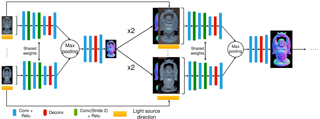
Figure 5. First two stages of the proposed multi-scale architecture. A first architecture, inspired by the PS-FCN method [7], takes as inputs the calibrated lighting directions and downsampled images, and outputs a low-resolution 3D normal map. The latter is then up-sampled and concatenated with lighting directions and higher-resolution images. A second architecture then infers higher-resolution normals, and this part of the process is repeated until the resolution of the original images is reached (network weights being shared by all scales).
