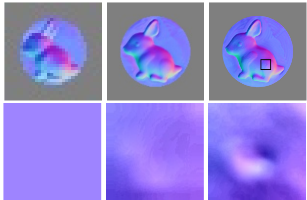
Figure 4. Multi-scale normal estimation at three different scales (bottom row is a contrast-enhanced zoom on the rectangle area). Low-detail geometry is reconstructed from the first levels. High-frequency details get refined as the scale increases.
