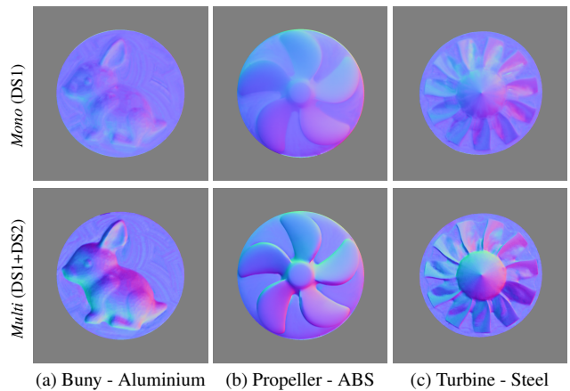
Figure 11. Visual comparison of the improvements brought by the combination of the new architecture and our new training set, on three objects from [29]. All three objects are much better reconstructed, although there the steel turbine remains challenging.
