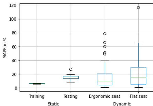
Figure 2. Model's errors (MAPE) between the experimental and predicted shear forces, averaged over 10s for the dynamic conditions.
