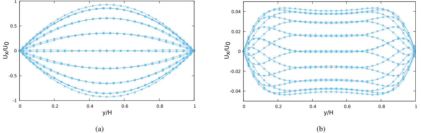
Figure 6: Newtonian oscillatory flow for (a) Re = 10 , \alpha = 1 and (b) Re = 10 , \alpha = 7 : numerical (symbols) and analytical (solid lines) velocity profiles at times t = n\pi/8 and n = \{0, \dots, 15\} .
