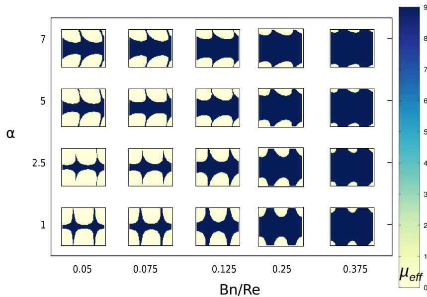
Figure 22: Space-time diagrams of dynamic viscosity during one period for each couple of dimensionless numbers \alpha , Bn/Re and n = 0.7 . For each subplot, the x-axis corresponds to the temporal evolution and the y-axis gives the position inside the channel. The blue part represents the “solid” behavior of the fluid while the white part represents the liquid part.
