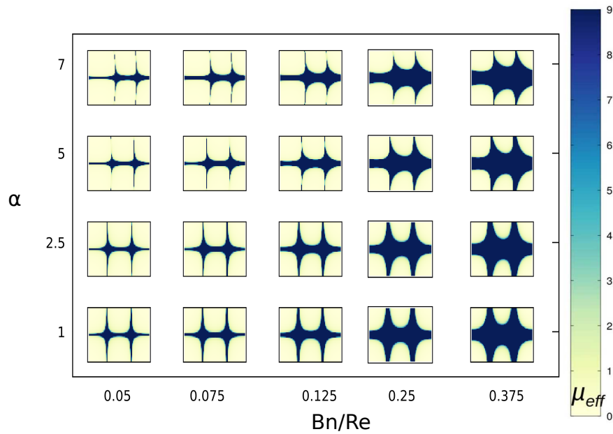
Figure 27: Space-time diagrams of dynamic viscosity during one period for each couple of dimensionless numbers \alpha , Bn/Re and n = 0.7 . For each subplot, the x-axis corresponds to the temporal evolution and the y-axis gives the position inside the channel. The blue part represents the “solid” behavior of the fluid while the white part represents the liquid part.
