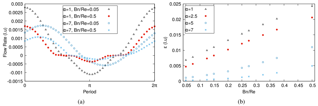
Figure 29: a) Flow rate over one period for n = 0.7 . b) Energy of harmonic frequency modes for various couples (\alpha, Bn/Re) and n = 0.7 .
