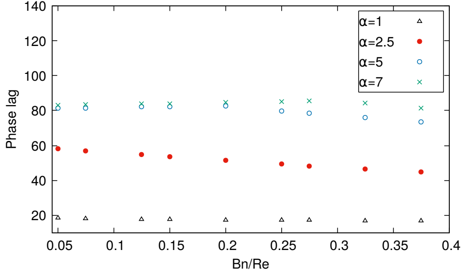
Figure 18: Phase lag between force and flow rate response for each couple of (\alpha, Bn/Re) and n = 1.3 .
