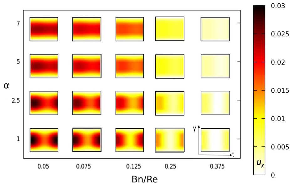
Figure 12: Space-time diagrams of the velocity during one period of oscillation for each couple of \alpha , Bn/Re and n=1.3 .
