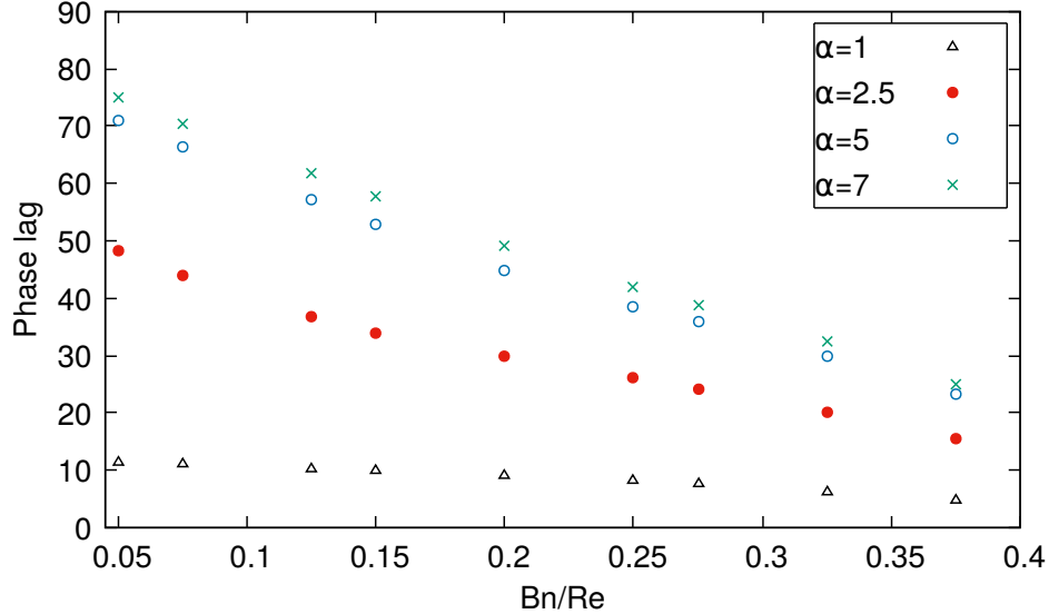
Figure 11: Phase lag (in degree) between the driving force and the flow rate for each couple of (\alpha, Bn/Re) and n = 1.3 .
