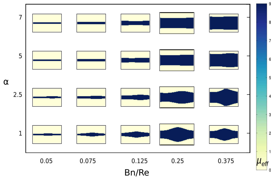
Figure 25: Space-time diagrams of dynamic viscosity during one period for each couple of dimensionless numbers \alpha , Bn/Re and n = 0.7 . For each subplot, the x-axis corresponds to the temporal evolution and the y-axis gives the position inside the channel. The blue part represents the “solid” behavior of the fluid while the white part represents the liquid part.
