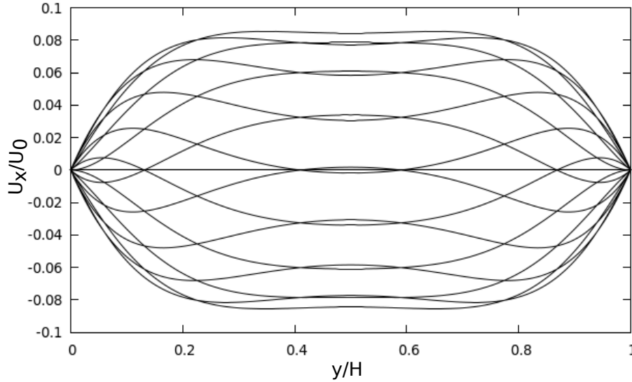
Figure 3: Analytical solution of the Newtonian oscillatory flow (Womersley flow) in a channel, for \xi_1 = 0 , \xi_2 = 1 , \alpha = 5 , Re = 0.1 at t = n\pi/8 for n = [0 : 15] , see equation (11).
