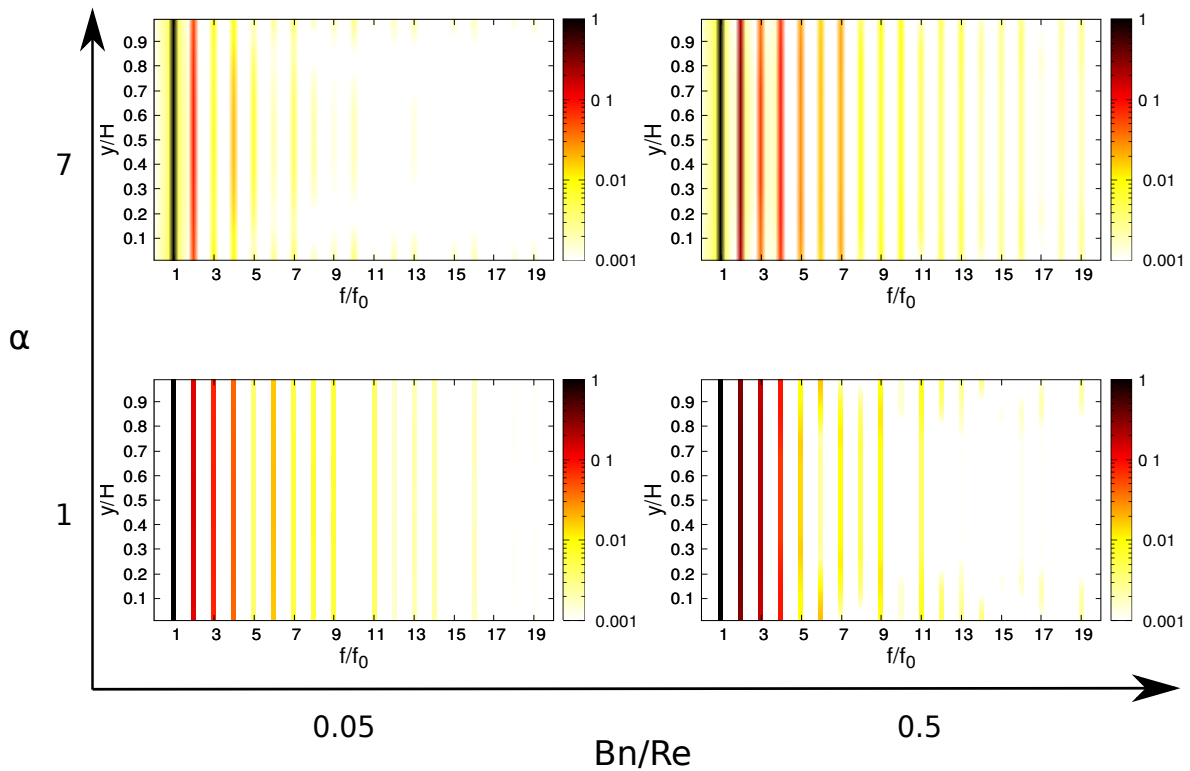
Figure 30: Space-time diagrams of the spectral energy on the velocity for each couple of \alpha, Bn/Re for n = 0.7 . The x-axis corresponds to the dimensionless frequency and the y-axis is the position inside the channel.
