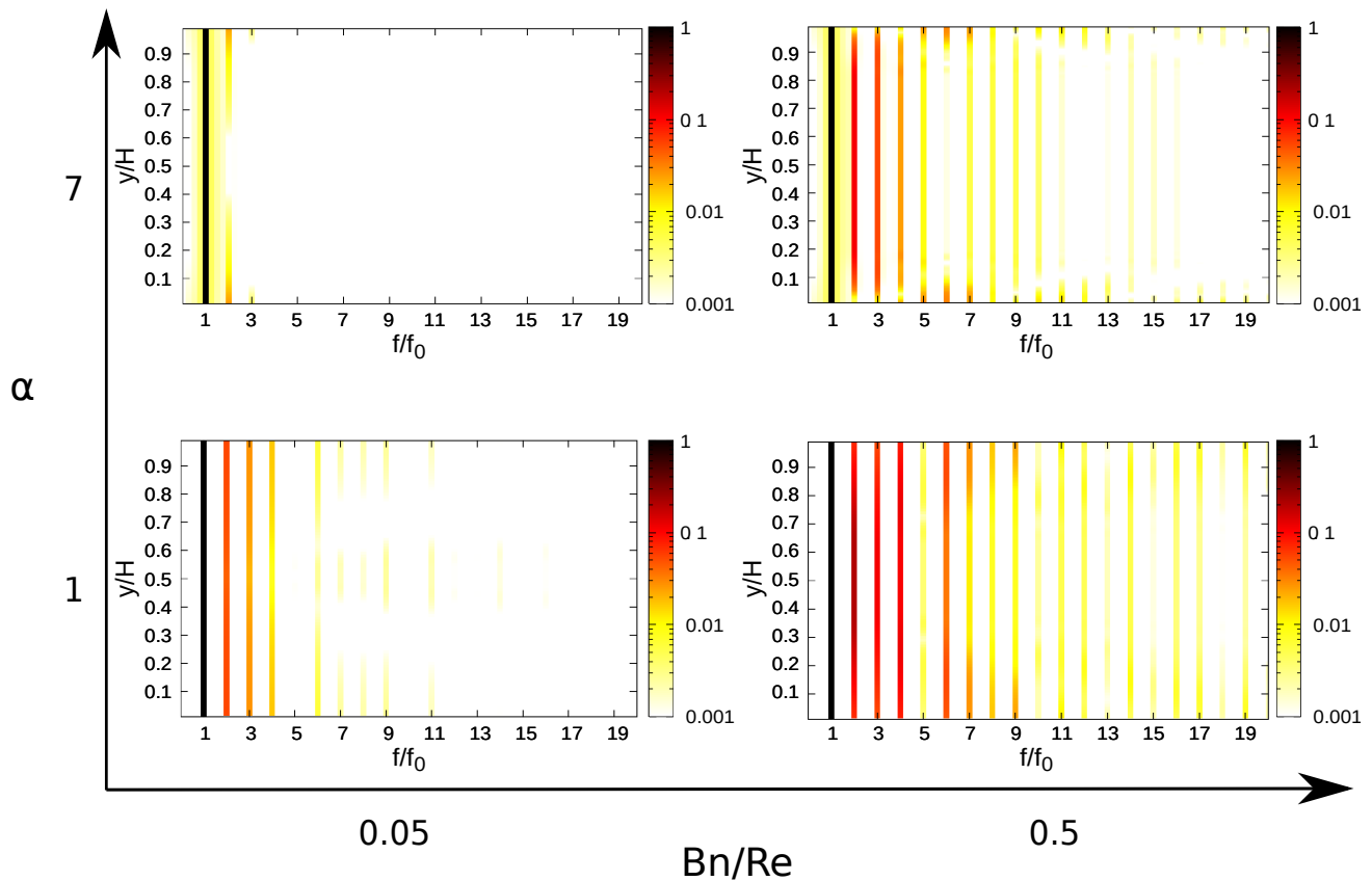
Figure 20: Space-frequency diagrams of the spectral energy on the velocity for each couple of \alpha , Bn/Re for n = 1.3 . The x-axis corresponds to the dimensionless frequency and the y-axis is the position inside the channel.
