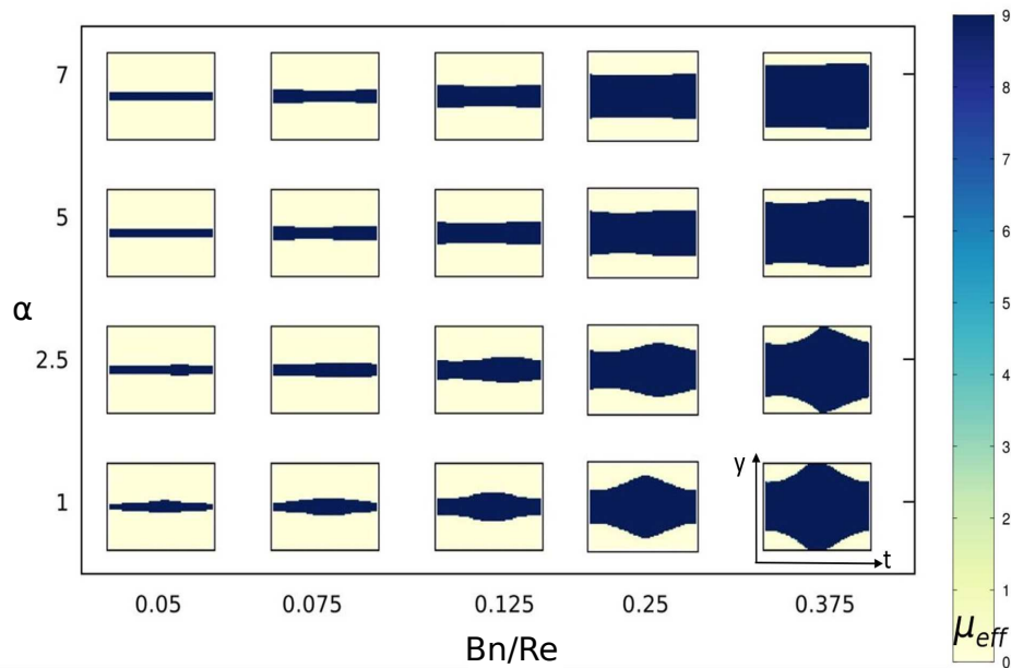
Figure 13: Space-time diagram of the dynamic viscosity during one period of oscillation for each couple of \alpha , Bn/Re and n=1.3 . For each subplot, the x-axis corresponds to the temporal evolution and the y-axis is the position inside the channel. The blue part represents the "solid" behavior of the fluid while the white part represents the liquid part.
