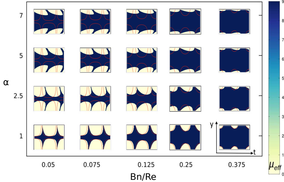
Figure 9: Space-time diagrams of dynamic viscosity during one period for each couple of dimensionless numbers \alpha , Bn/Re and n = 1.3 . For each subplot, the x-axis corresponds to the temporal evolution and the y-axis gives the position inside the channel. The blue part represents the “solid” behavior of the fluid while the white part represents the liquid part. The red line corresponds to the position of the interface y_{i0}(t)
