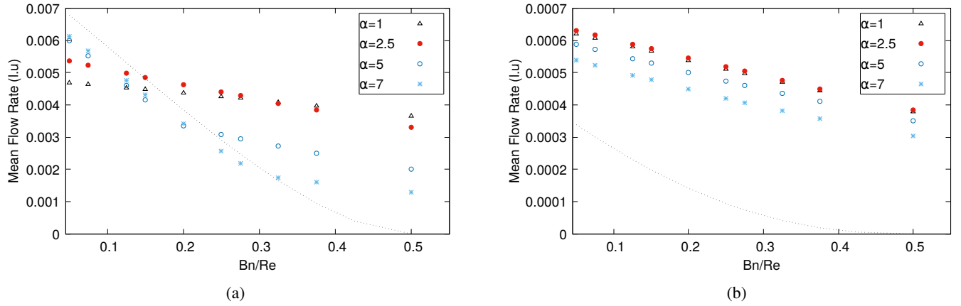
Figure 17: a) Mean flow rate for each couple of (\alpha, Bn/Re) and n = 1.3 . b) Mean flow rate for each couple of (\alpha, Bn/Re) and n = 0.7 . dotted line: Flow rate for Poiseuille Flow.
