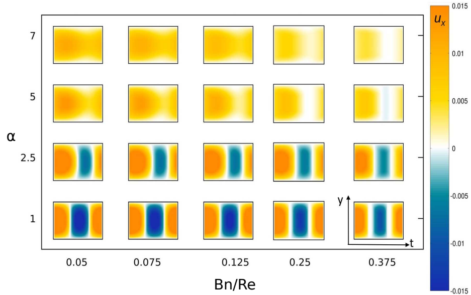
Figure 15: Space-time diagram of the velocity during one period of oscillation for each couple of \alpha, Bn/Re and n=1.3 (high amplitude, low mean flow). For each subplot, the x-axis corresponds to the temporal evolution and the y-axis is the position inside the channel.
