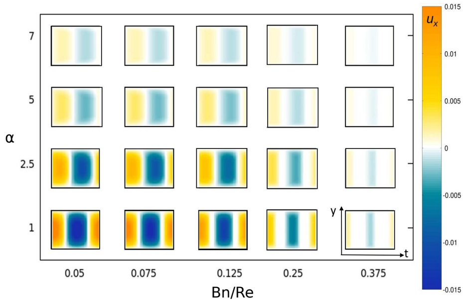
Figure 8: Space-time diagram of the velocity field during one period for each couple of dimensionless numbers \alpha , Bn/Re and n = 1.3 . The velocity magnitude is indicated by the color bar. For each subplot, the x-axis corresponds to the temporal evolution and the y-axis gives the position inside the channel.
