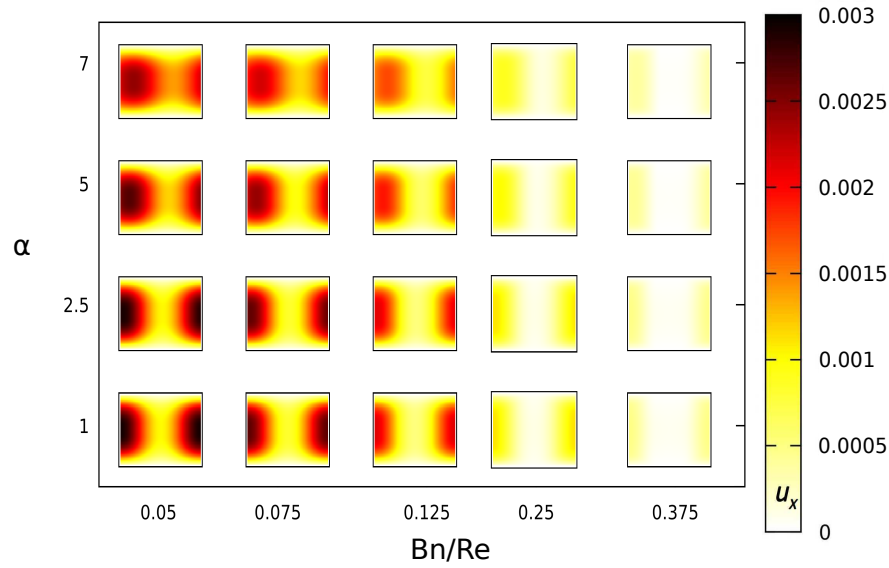
Figure 24: Space-time diagram of the velocity field during one period for each couple of dimensionless numbers \alpha , Bn/Re and n = 0.7 . The velocity magnitude is indicated by the color bar. For each subplot, the x-axis corresponds to the temporal evolution and the y-axis gives the position inside the channel.
