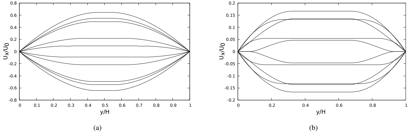
Figure 7: Velocity profile for n = 2\pi/10 , for n being an integer number between 0 and 9 a) Re = 0.1 , Bn/Re = 0.05 , \alpha = 1 and n = 1.3 b) Re = 0.1 , Bn/Re = 0.05 , \alpha = 7 and n = 1.3 .
