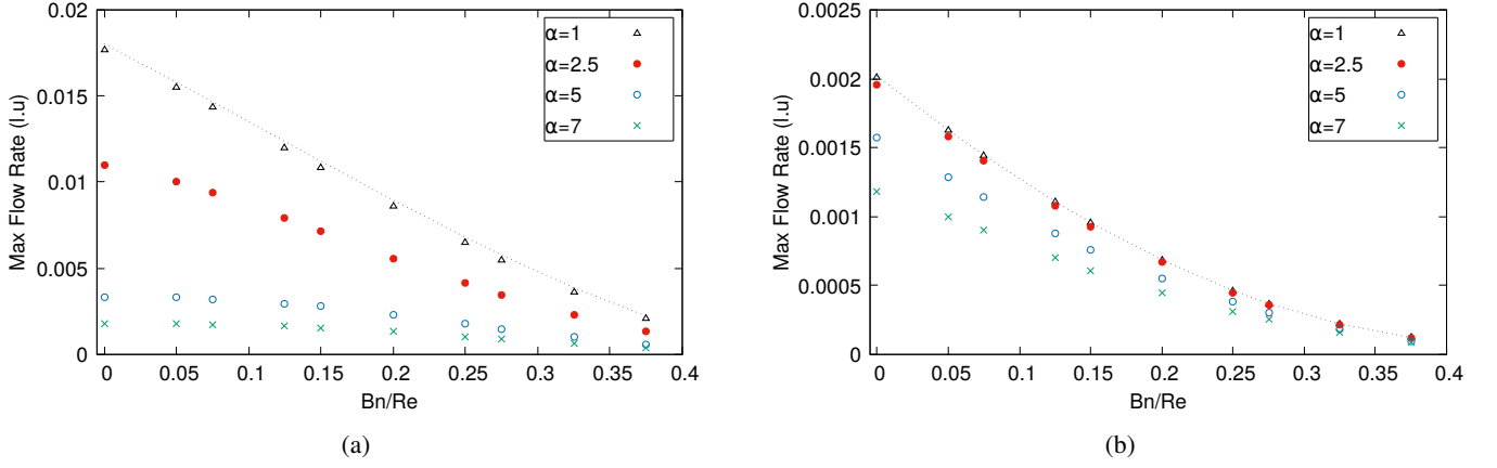
Figure 10: Maximal flow rate in lattice units (l.u.) for each couple of (\alpha, Bn/Re) and (a) n=1.3 and (b) n=0.7 . Dotted line: Flow rate for Poiseuille Flow.
