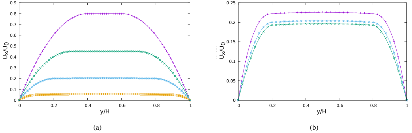
Figure 5: Velocity profiles a) Re = 10 , n = 1 and different Bn , Purple: Bn = 1 , Green: Bn = 2 , Blue: Bn = 3 , Yellow: Bn = 4 , b) Re = 10 , Bn = 3 , Purple: n = 0.7 , Blue: n = 1 , Green: n = 1.3 . The lines represent the analytical solutions and the symbols the numerical ones.
