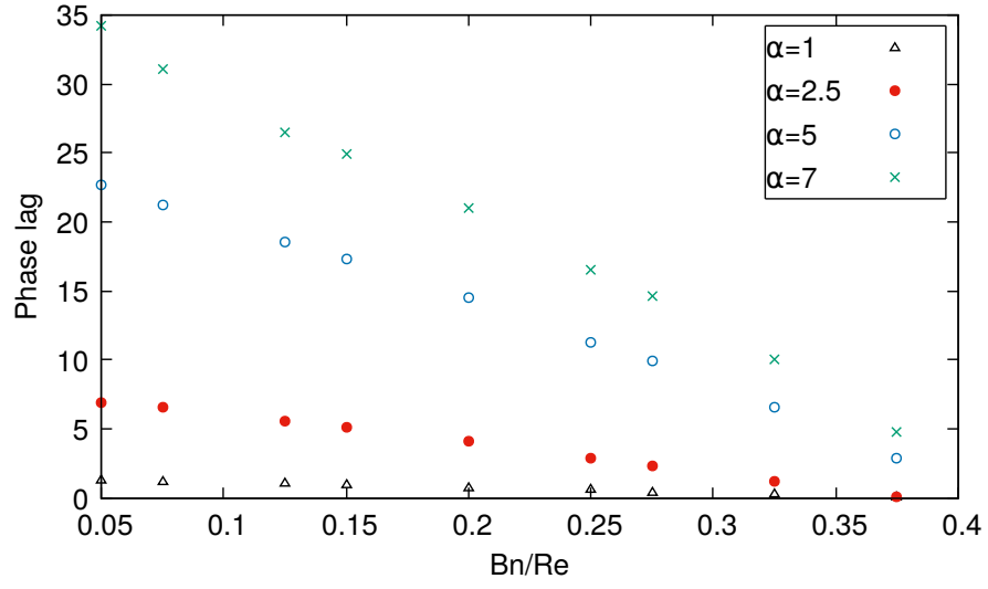
Figure 23: Phase lag (in degree) between the driving force and the flow rate for each couple of (\alpha, Bn/Re) and n = 0.7 .
