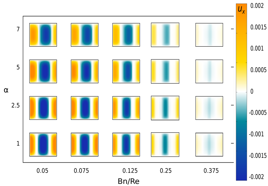
Figure 21: Space-time diagram of the velocity field during one period for each couple of dimensionless numbers \alpha , Bn/Re and n = 0.7 . The velocity magnitude is indicated by the color bar. For each subplot, the x-axis corresponds to the temporal evolution and the y-axis gives the position inside the channel.
