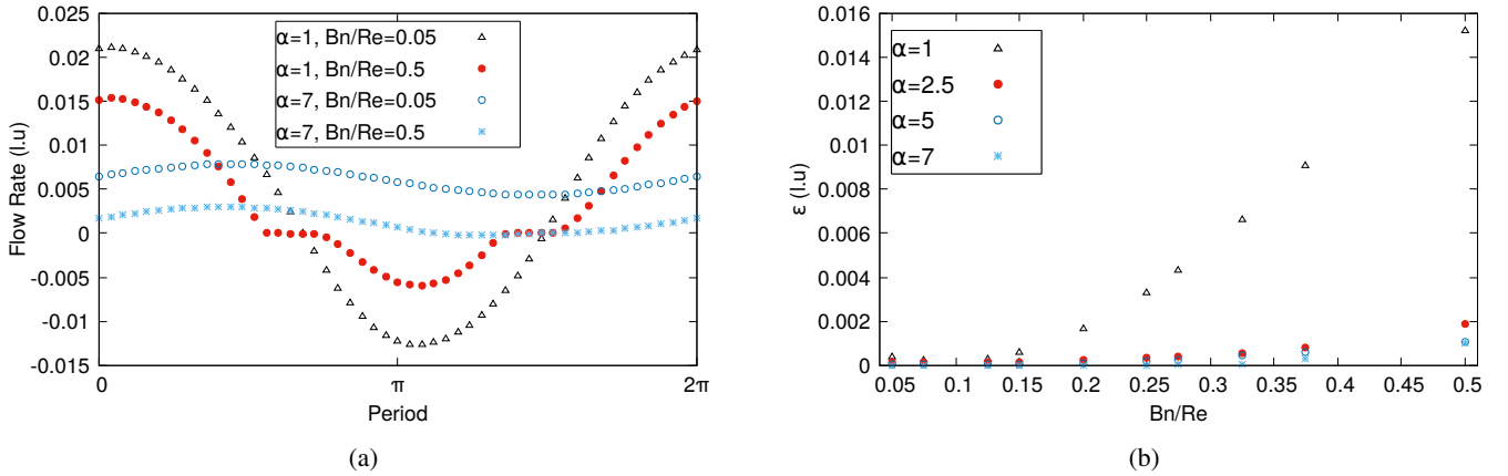
Figure 19: a) Flow rate over one period for n = 1.3 . b) Energy of harmonic frequency modes for various couples (\alpha, Bn/Re) and n = 1.3 .
