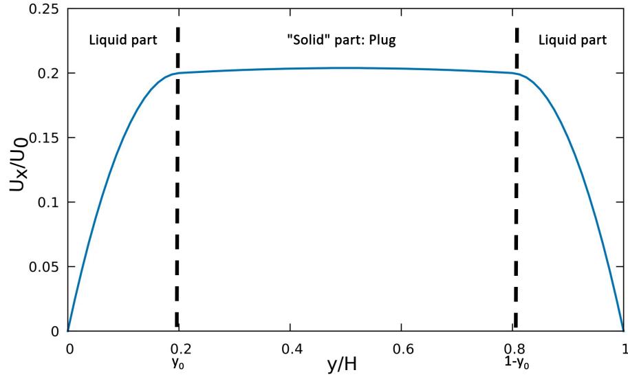
Figure 2: Analytical solution for the Herchel-Bulkley flow driven by a constant body force, Bn/Re = 3/10 , n = 1 and \mu_r = 2500 see equation (II B 1).
