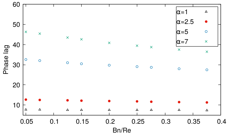
Figure 28: Phase lag between force and flow rate response for each couple of (\alpha, Bn/Re) and n = 0.7 .
