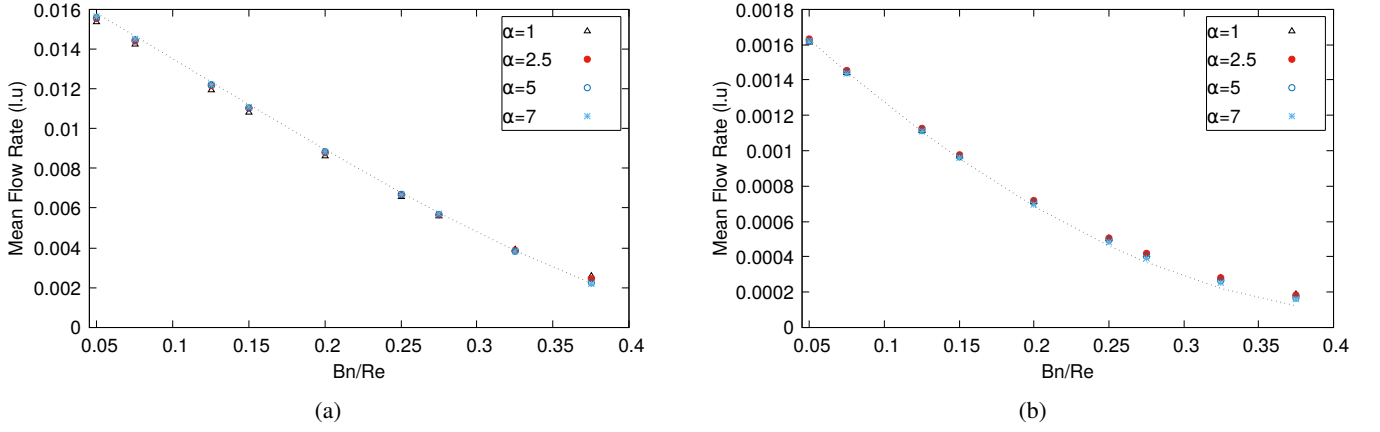
Figure 14: Mean flow rate for each couple of (\alpha, Bn/Re) and (a) n = 1.3 and (b) n = 0.7 . Dotted line: Flow rate for Poiseuille Flow
