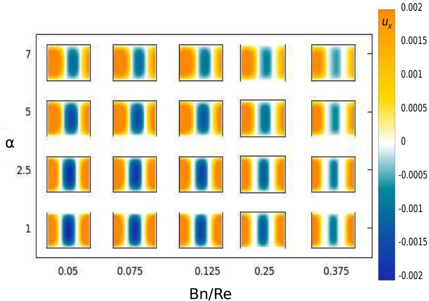
Figure 26: Space-time diagram of the velocity field during one period for each couple of dimensionless numbers \alpha , Bn/Re and n = 0.7 . The velocity magnitude is indicated by the color bar. For each subplot, the x-axis corresponds to the temporal evolution and the y-axis gives the position inside the channel.
