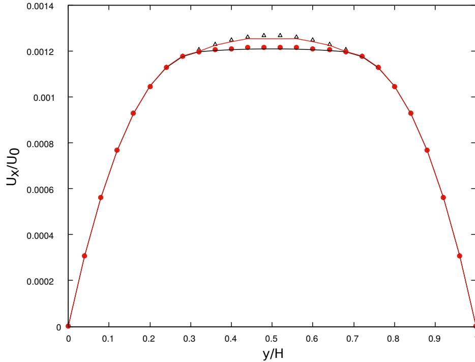
Figure 4: Impact of the viscosity ratio on the velocity profile for Re = 0.1 , Bn/Re = 0.15 , n = 0.7 , \triangle : \mu_r = 500 , \bullet : \mu_r = 1500 , black line: \mu_r = 2500 and red line: \mu_r = 3500 .
