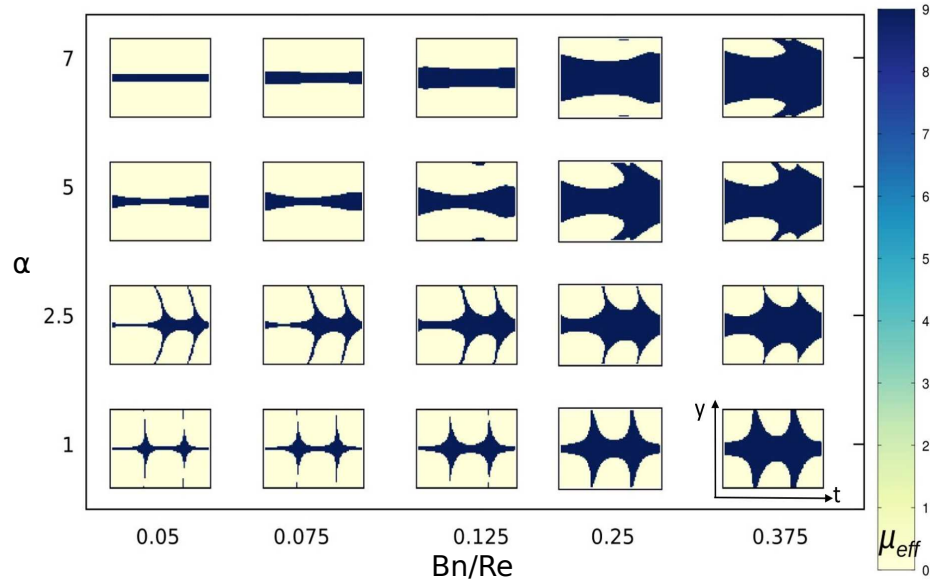
Figure 16: Space-time diagram of the dynamic viscosity during one period of oscillation for each couple of \alpha , Bn/Re and n=1.3 (high amplitude, low mean flow). For each subplot, the x-axis corresponds to the temporal evolution and the y-axis is the position inside the channel. The blue part represents the "solid" behavior of the fluid while the white part represents the liquid part.
