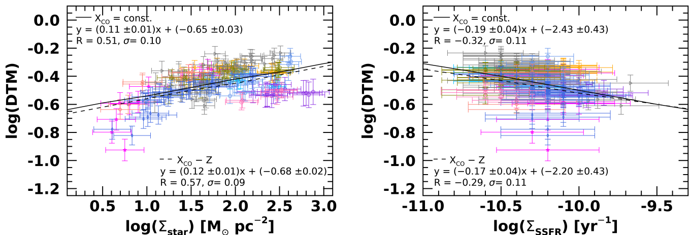
Fig. 10: Logarithm of dust-to-metal ratio as a function of logarithm of \Sigma_{\text{star}} (left panel) and of \Sigma_{\text{SSFR}} (right panel). Data points refer to constant X_{\text{CO}} , fit lines to both assumptions on X_{\text{CO}} (see legend in Fig. 7 and Table 5). Symbols are same as Fig. 2.
