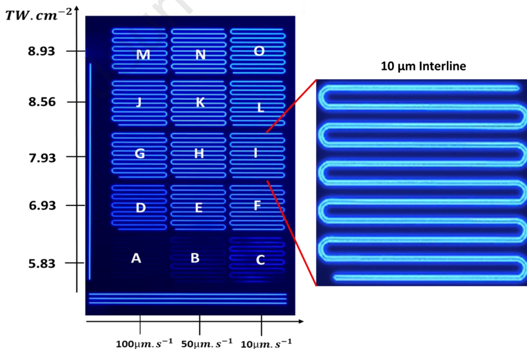
Figure 4: Laser/glass interaction matrix showing luminescent square patterns versus laser peak irradiance and sample motion velocity (wide-field fluorescence micrograph under
