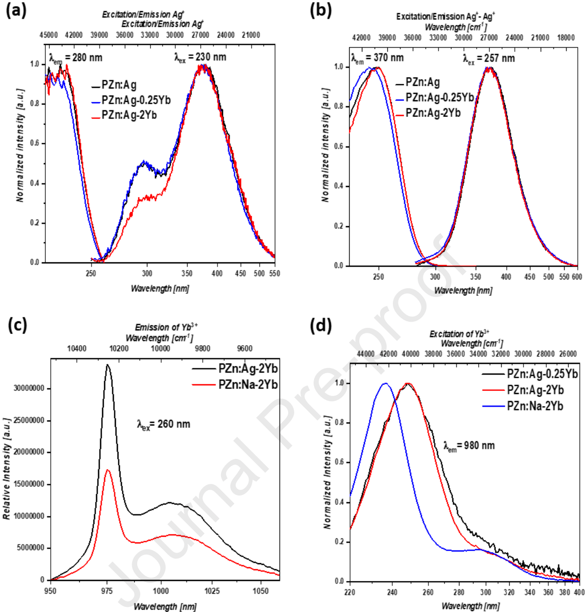
Figure 2 : Excitation and emission spectra of Ytterbium doped and undoped PZn4Ag glass. (a) Excitation/emission spectra of Ag^+ ions; (b) Excitation/emission spectra of Ag^+-Ag^+ ; (c) emission spectrum of Yb^{3+} ions for 260 nm excitation; (d) Excitation spectrum of Yb^{3+} ions for 980 nm emission.
