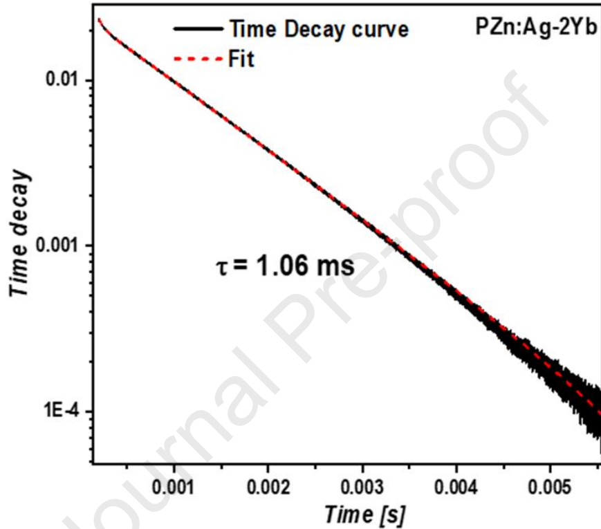
Figure 3: Lifetime of \text{Yb}^{3+} in the PZn:Ag-2Yb glass (excitation at 940 nm).
