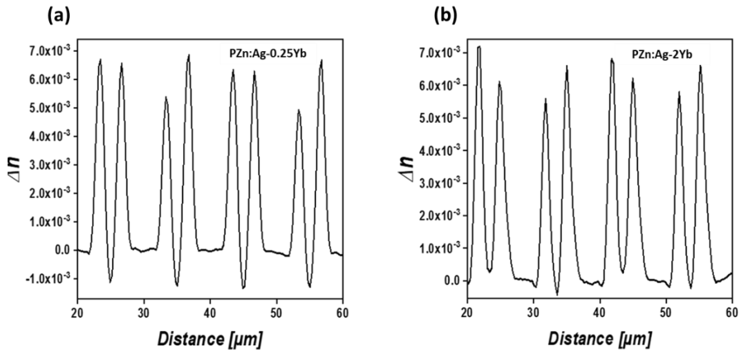
Figure 5: Profile of the refractive index change of four laser inscription passes, depicting a positive double-track distribution (up to 7 \times 10^{-3} ) perfectly co-located to that of the laser-
