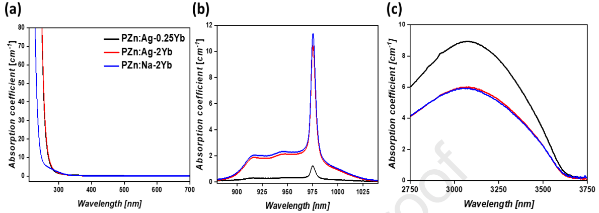
Figure 1: Absorption spectra of \text{Yb}^{3+} -doped and \text{Yb}^{3+} -free silver containing PZn pristine glass. (a) Absorption edge in UV range; (b) Absorption band of \text{Yb}^{3+} ; (c) Absorption band of P-OH.
