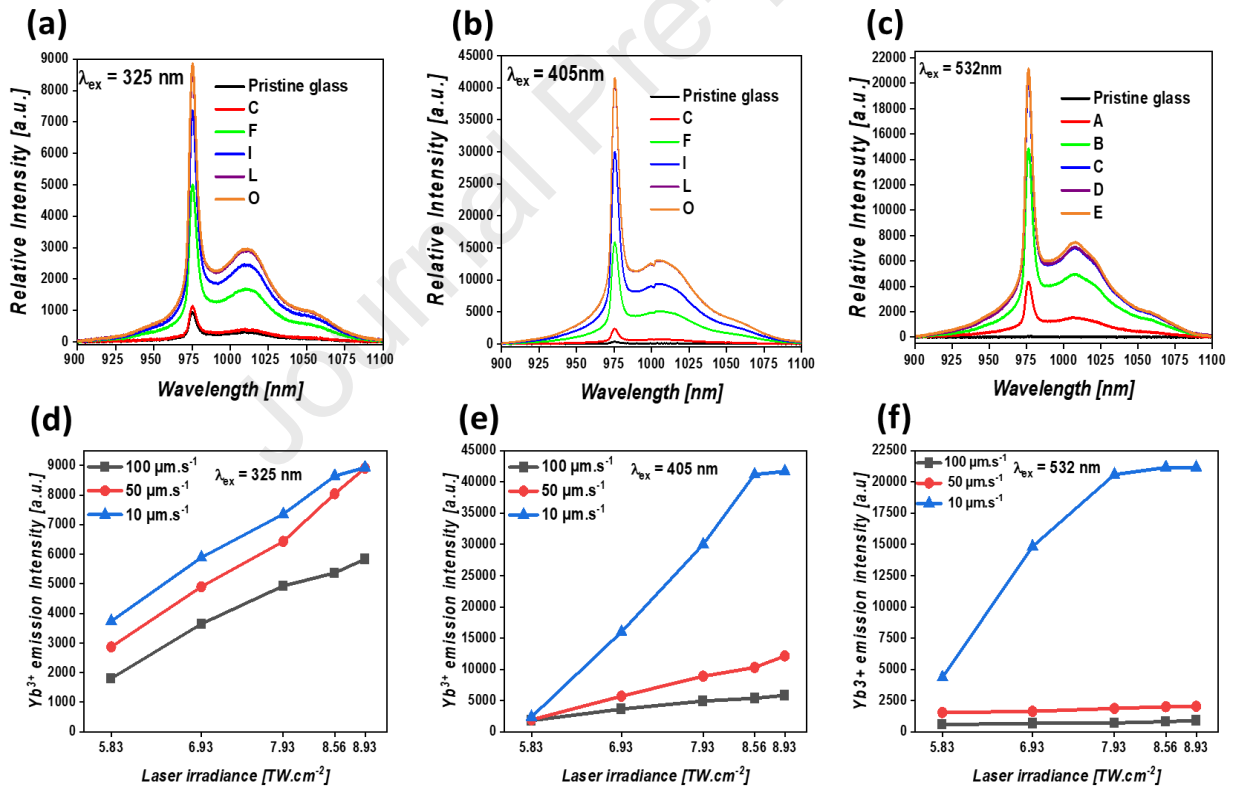
Figure 7 : (a, b, c) Confocal near-IR fluorescence emission spectra of the PZn:Ag-2Yb sample from the laser-created patterns inscribed at 10 \mu\text{m}\cdot\text{s}^{-1} from Fig. 2, for excitation wavelengths at 325 nm, 405 nm, and 532 nm, respectively. (d, e, f) Associated zero-phonon line amplitudes spectra of the \text{Yb}^{3+} ions for all the patterns of the interaction matrix from Fig. 2.
