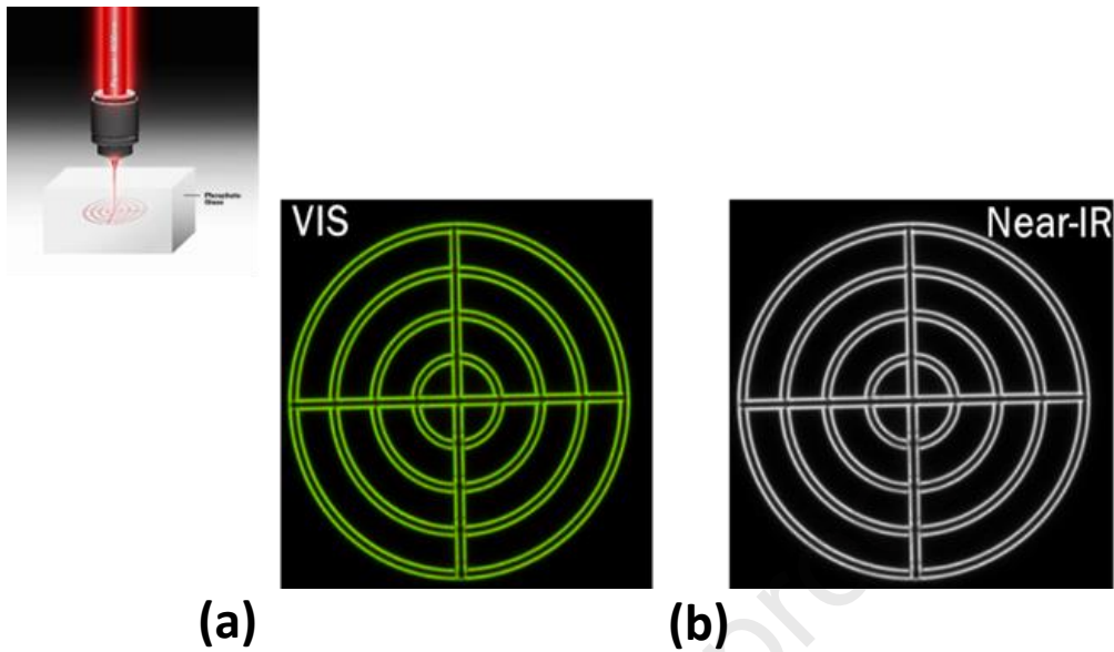
Figure 8: Confocal image of a multi-scale photonic architecture showing sub-diffraction features, corresponding to a fluorescent target for high-resolution calibration optical standard for confocal fluorescence microscopy, for excitation at 473 nm. (a) Emission of the silver clusters integrated into the visible range over the 500-700 nm range; (b) co-localized near-IR emission of the \text{Yb}^{3+} ions integrated over the 920-1050 nm range. Scale: concentric circles show radii with a 5 \mu\text{m} increment.
