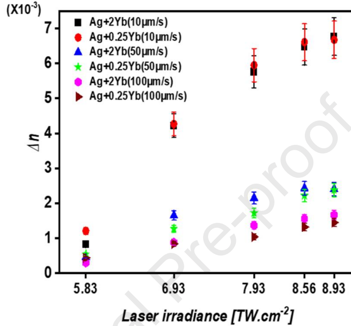
Figure 6: Amplitude of the positive refractive index modification \Delta n versus laser irradiance, for different velocities and associated a cumulated number of pulse, for both the PZn:Ag-0.25 and PZn:Ag-2Yb glasses, showing the increase and progressive saturation behavior of such \Delta n modification with the deposited dose by laser irradiation.
