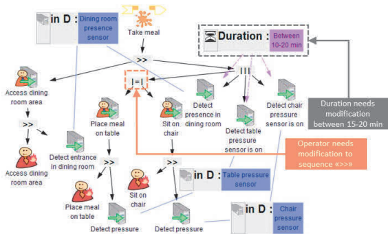
Fig. 10: Task model modified for taking meal events.
