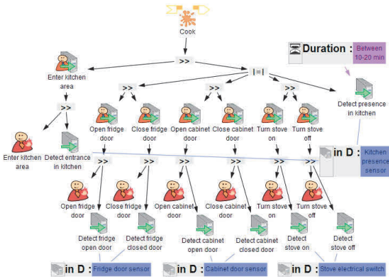
Fig. 3: Tasks to subroutine "cook"
