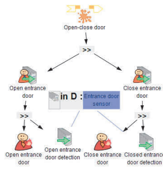
Fig. 4: Tasks to subroutine "open-close door"
