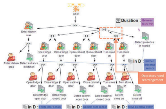
Fig. 11: Task model modified for cooking events.
