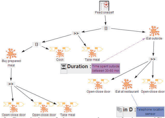
Fig. 2: Description of the user tasks to “feed oneself” with HAMSTERS-XL notation.
