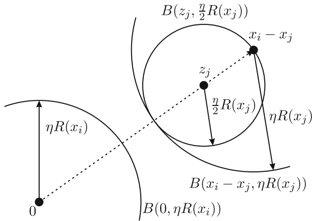
Fig. 2 Sketch of Construction
