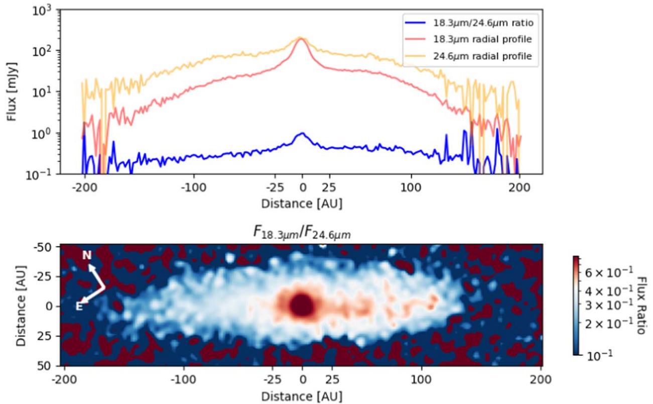
Figure 4. Top: radial surface brightness profile of the 18.3\ \mu\text{m} band and 24.6\ \mu\text{m} \beta Pic images from T-ReCS Telesco et al. (2005) imaging and ratio of the surface brightness profile. Bottom: flux ratio between the 18.3\ \mu\text{m} band and 24.6\ \mu\text{m} from T-ReCS imaging (Telesco et al. 2005). The red color indicates regions in which the 18.3\ \mu\text{m} emission is relatively bright compared with the 24.6\ \mu\text{m} emission. The bottom panel shows that the 18\ \mu\text{m} flux originates from regions (red colors) close to central star (within 10'' ) while the 24\ \mu\text{m} flux originates from more distant regions in the disk (blue).
