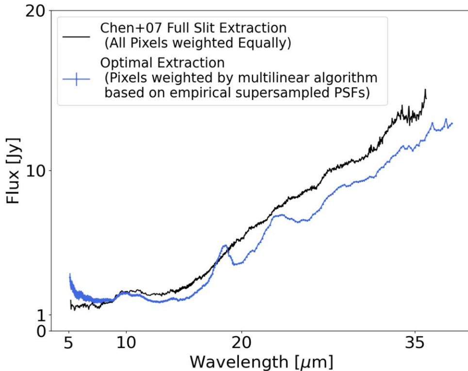
Figure 3. The \beta Pic IRS spectrum showcasing the newly discovered 18 \mu\text{m} feature and a 23 \mu\text{m} feature with larger line-to-continuum ratio than previously reported by Chen et al. (2007). The optimal extraction (this work) is in blue, while the full-slit extraction published in Chen et al. (2007) is in black. The uncertainties for the spectrum extracted with AdOpt are on average at the 1% level. The Chen+07 spectrum reduced using a full-slit extraction has fringes.
