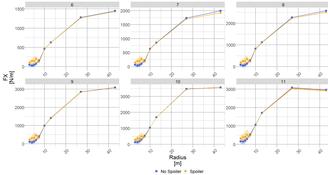
Figure 13. The blue square (blue ■) shows the force normal to the rotor plane evolution along the blade radius without spoiler, and the orange dot (orange ●) shows the normal force to the rotor plane evolution along the blade radius with spoiler. Each subplot shows the results for a wind speed ( \text{m s}^{-1} ) whose value is given in the title.
