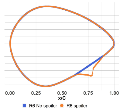
Figure 1. Overimposed aerofoil shapes at radial position R6 ( r/R = 13\% ): the blue square (blue ■) shows the no-spiller coordinates while the orange dot (orange ●) shows the spoiler coordinates.
