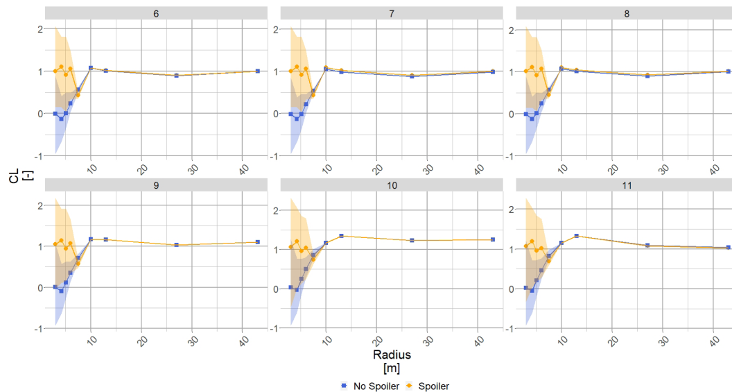
Figure 11. The blue square (blue ■) shows the C_L evolution along the blade radius without spoiler, and the orange dot (orange ●) shows the C_L evolution along the blade radius with spoiler. Each subplot shows the results for a wind speed ( \text{m s}^{-1} ) whose value is given in the title.
