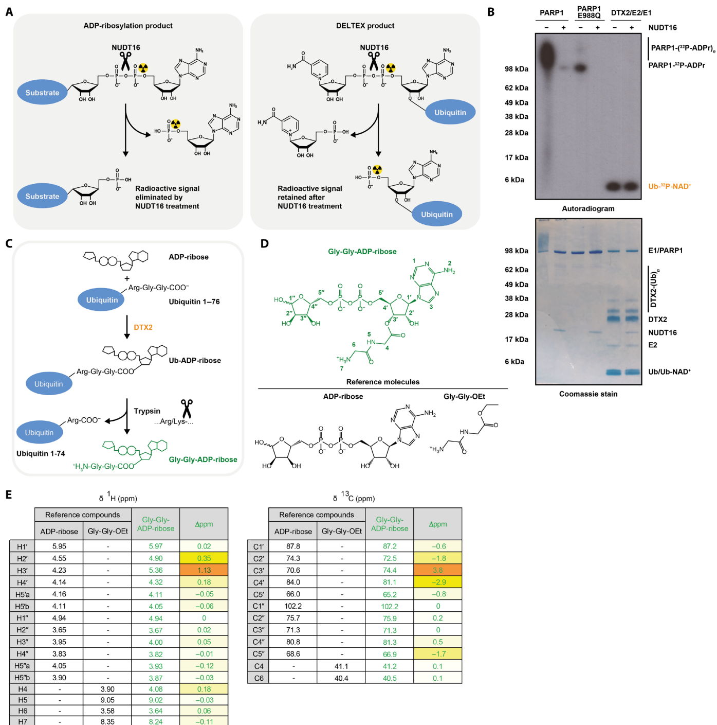
Fig. 2. DTX E3s catalyze conjugation of Ub to the 3' hydroxyl of \text{NAD}^+ /ADP-ribose. (A) Schematic diagram of expected NUDT16 cleavage specificity. NUDT16 treatment eliminates radioactivity from a ^{32}\text{P} - \text{NAD}^+ -labeled protein if it is attached to the dinucleotide via C1'' but not when it is attached to the adenine-proximal ribose. (B) Poly(ADP-ribosyl)ated PARP1 WT, mono(ADP-ribosyl)ated PARP1 E988Q, and the DTX product were created by incubating the relevant components with \text{NAD}^+ and then treated or not with NUDT16. The samples were analyzed on an SDS-PAGE gel, which is then visualized by Coomassie staining and autoradiography. NUDT16 reverses PARP1/PARP1 E988Q automodification but has no effect on the DTX2-catalyzed Ub- \text{NAD}^+ adduct, consistent with the adenine-proximal Ub attachment. (C) Flowchart of Gly-Gly-ADP-ribose generation. The DTX reaction followed by trypsin digestion results in ADP-ribose attached to the tryptic Ub remnant Gly-Gly-. Trypsin cleavage specificity is indicated. (D) Chemical formulas of Gly-Gly-ADP-ribose and reference molecules used in NMR. (E) NMR localization of the Gly-Gly remnant to the 3' hydroxyl group of the proximal ribose of ADP-ribose based on the largest shifts ( \Delta\text{ppm} ) in \delta^1\text{H} and ^{13}\text{C} values in these positions. For ADP-ribose and Gly-Gly-ADP-ribose, \delta^1\text{H} and ^{13}\text{C} values are provided only for the major \beta anomer (full data and explanation in the Supplementary Materials).
