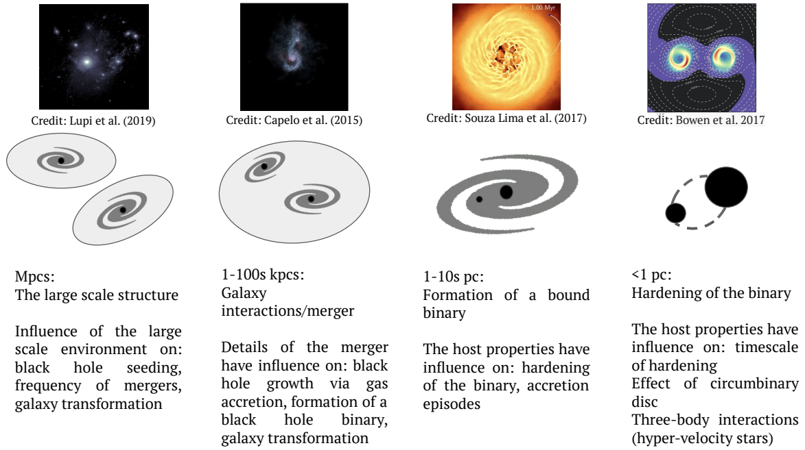
Figure 2.1: A schematic view of the complex and multi-scale processes affecting the formation of a hard MBH binary system. Figure credit: Silvia Bonoli and Alessandro Lupi.
