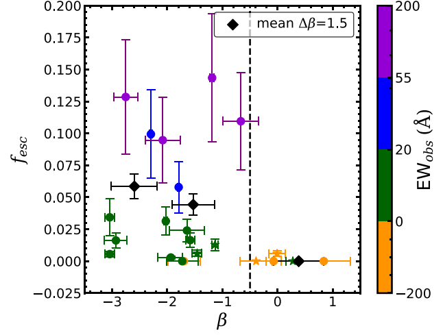
Figure 11. The Ly \alpha escape fraction as a function of UV spectral slope ( \beta ). The colour coding and markers are the same as in Fig. 7. The black dashed vertical line is set as a limit for LAEs. All LAEs have slopes bluer than -0.5 . There is large variance in beta for similar f_{\text{esc}} , perhaps suggesting bursty star formation. The black diamonds are mean values of the escape fraction in bins of \Delta\beta = 1.5 . The error bars are calculated by propagating the statistical uncertainty of each datum. One object was excluded due to highly uncertain \beta from low S/N continuum.
