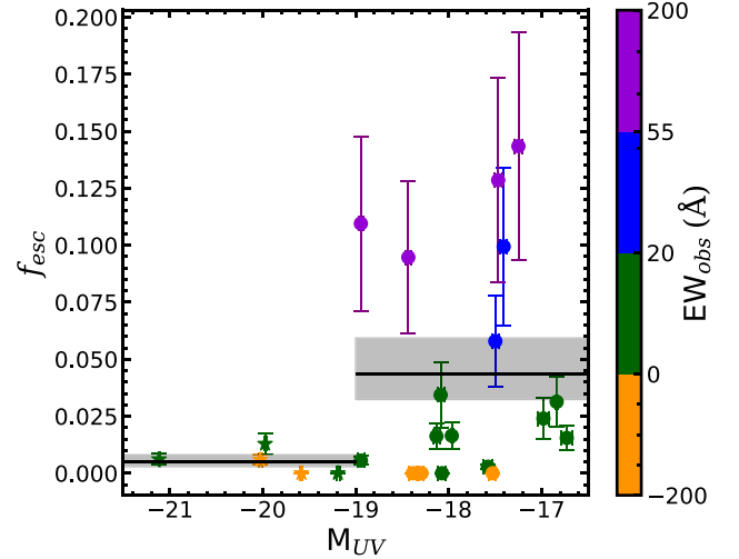
Figure 8. The Ly \alpha escape fraction as a function of absolute UV magnitude ( M_{UV} ). The colour coding and markers are the same as in Fig. 7. The mean escape fraction of the dwarf galaxies ( 4.3^{+1.6}_{-1.1} per cent) and the more massive galaxies ( 0.5^{+0.3}_{-0.2} per cent) are displayed with shaded black regions denoting the propagated uncertainty in the individual galaxies. However, the bright galaxy sample has only five galaxies and is therefore uncertain.
