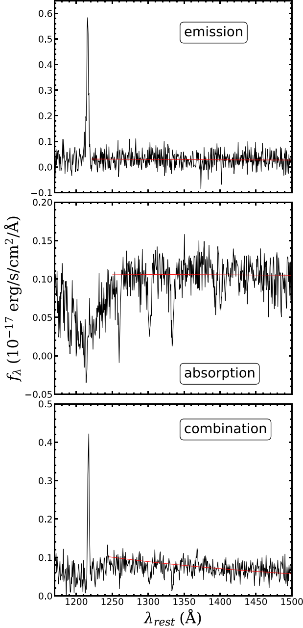
Figure 1. Three example spectra from our sample of galaxies. The red line is the continuum fit for each spectrum. The fitting method is described in Section 3. Top: An example of an ‘emission’ spectrum where we have Ly \alpha in emission only. Middle: An example of an ‘absorption’ spectrum. Bottom: An example of a ‘combination’ spectrum where we see absorption and emission around Ly \alpha .
