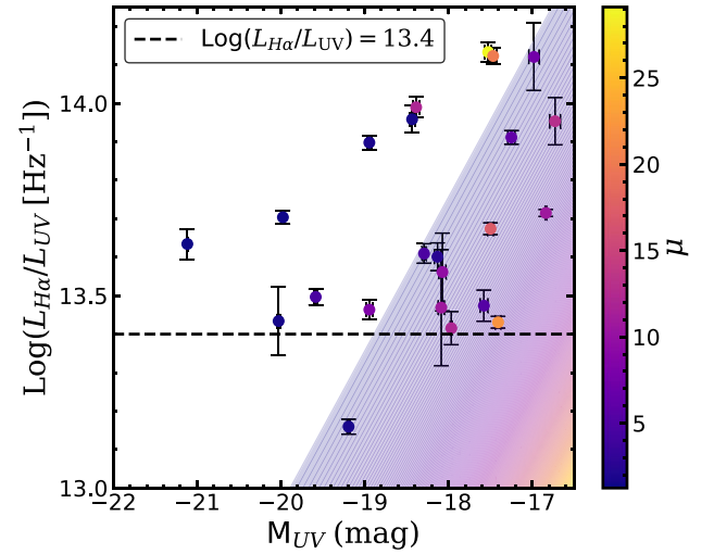
Figure 3. Plotted is the \log(L_{H\alpha}/L_{UV}) versus denlensed absolute UV magnitude. Points are colour coded according to each galaxy’s magnification. The black dashed line at \log(L_{H\alpha}/L_{UV}) = 13.4 denotes our completeness limit for the sample. The angled coloured space demonstrates the 3\sigma H\alpha sensitivity limit of our detector colour coded according to magnification. Errors on M_{UV} do NOT include uncertainties on the lens model.
