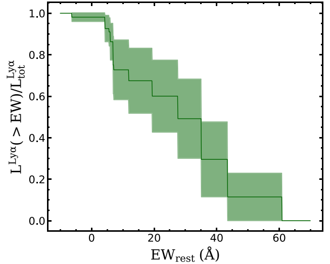
Figure 6. The integrated \text{Ly}\alpha luminosity density as a function of EW. The uncertainty is given by the shaded green regions. We find that about 60 per cent of the integrated luminosity density comes from galaxies with \text{EW}_{\text{Ly}\alpha} > 20 Å.
