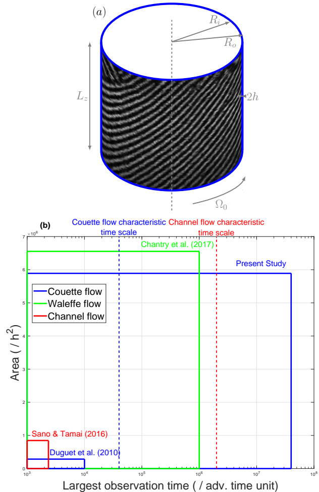
FIG. 1. Schematic of experimental apparatus (top); typical test section sizes and time scales covered in previous studies when compared to the present experiment (bottom). Note that the observation time is defined as the maximum time over which the evolution of a flow pattern can be investigated in a co moving frame. It hence does not necessarily coincide with (and often is far shorter than) the recording time.
