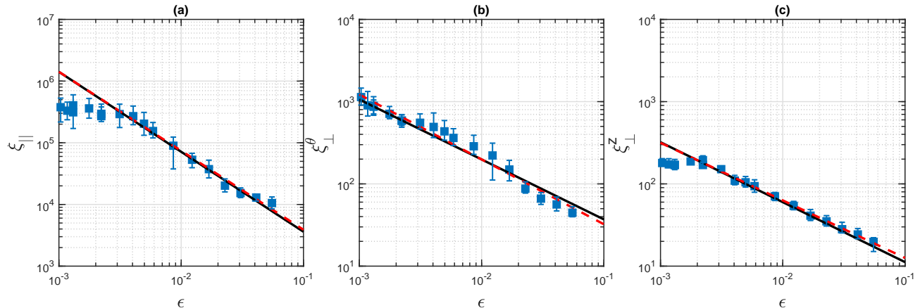
FIG. 4. Correlation exponents at the phase transition. Dependence of correlation time (panel (a): \xi_{\parallel} ) and correlation lengths (panel (b): \xi_{\perp}^{\theta} ; panel (c): \xi_{\perp}^z ) on control parameter \epsilon . In each panel the red dashed line corresponds to the best fit (panel (a): \xi_{\parallel} \sim \epsilon^{-\nu_{\parallel}} with \nu_{\parallel} = 1.28 ; panel (b): \xi_{\perp}^{\theta} \sim \epsilon^{-\nu_{\perp}^{\theta}} with \nu_{\perp}^{\theta} = 0.79 ; panel (c): \xi_{\perp}^z \sim \epsilon^{-\nu_{\perp}^z} with \nu_{\perp}^z = 0.70 ) and black solid lines correspond to the theoretical predictions for the (2+1)DP universality class ( \nu_{\parallel} = 1.296 , \nu_{\perp}^{DP} = 0.729 ).
