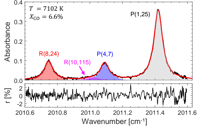
Fig. 4 Typical fit of the CO absorption spectrum between 2010.6 and 2011.6 \text{cm}^{-1} .
