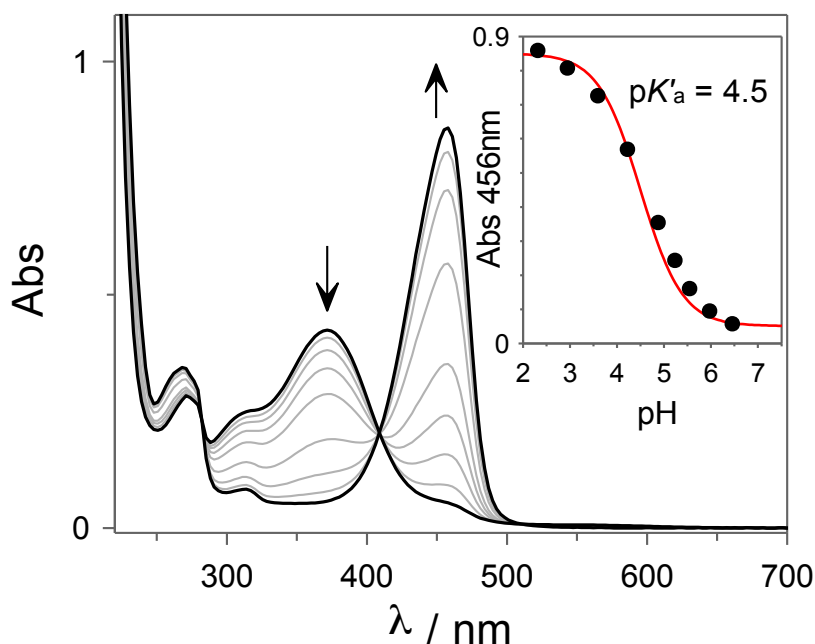
Figure 5 – UV-Vis absorption spectra of equilibrated solutions of 1 (18 \mu\text{M} ) in the presence of 1 equivalent of CB7 in 10 mM of aqueous citrate buffer at different pH values. Inset: Absorbance at 456 nm as a function of pH.
