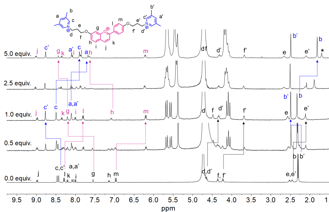
Figure 4 – 1 H NMR spectra of 2 (1.5 mM) in the presence of increasing concentrations of CB7 in D 2 O at pH = 1 ([DCl] = 0.1 M). Contrary to 1 , in this case the slow exchange between free and complexed species with defined stoichiometry and co-conformation leads to the observation of sharper signals in the 1 H NMR spectra. * denotes a minor impurity.
