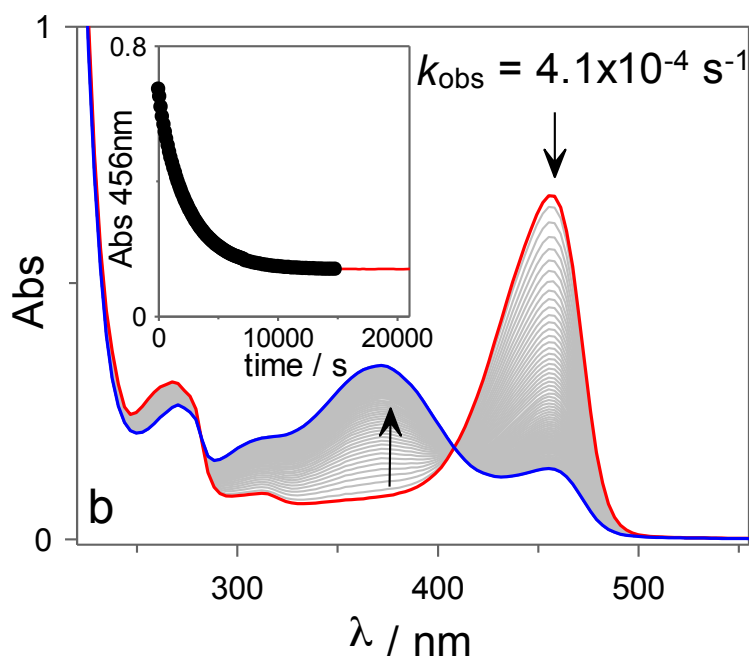
Figure 6 –(a) UV-Vis absorption spectra observed upon irradiation (365 nm) of an aqueous solution of 1 (18 \mu\text{M} ) in the presence of 1 equiv. of CB7 at pH = 5.4 (10 mM of citrate buffer). (b) Thermal recovery from the photostationary state at 20 ^{\circ}\text{C} .
