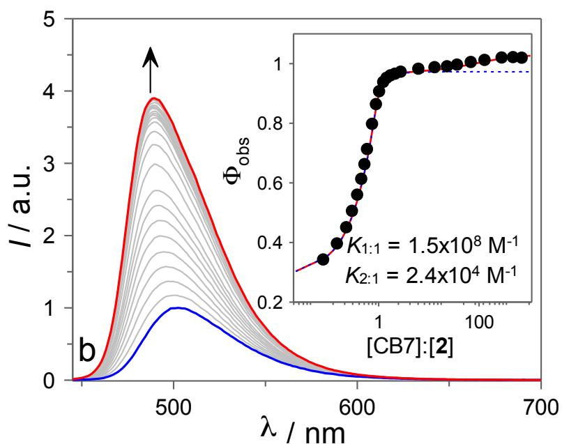
Figure 3 – (a) UV-Vis absorption spectra of flavylum 2 (15 \mu\text{M} ) in the presence of increasing concentrations of CB7 in water at \text{pH} = 1 . Inset: Absorbance at 462 nm on increasing amount of CB7; (b) Emission spectra of flavylum 2 (0.5 \mu\text{M} ) in the presence of increasing concentrations of CB7 in water at \text{pH} = 1 ( \lambda_{\text{ex}} = 430 nm, excitation slits = 9 nm, emission slits = 4.5 nm). Inset: observed fluorescence quantum yield on increasing amount of CB7. Traced blue line is the fitting to a 1:1 model ( K_{1:1} = 1.5 \times 10^8 \text{M}^{-1} ) and the red line to a sequential 2:1 model.
