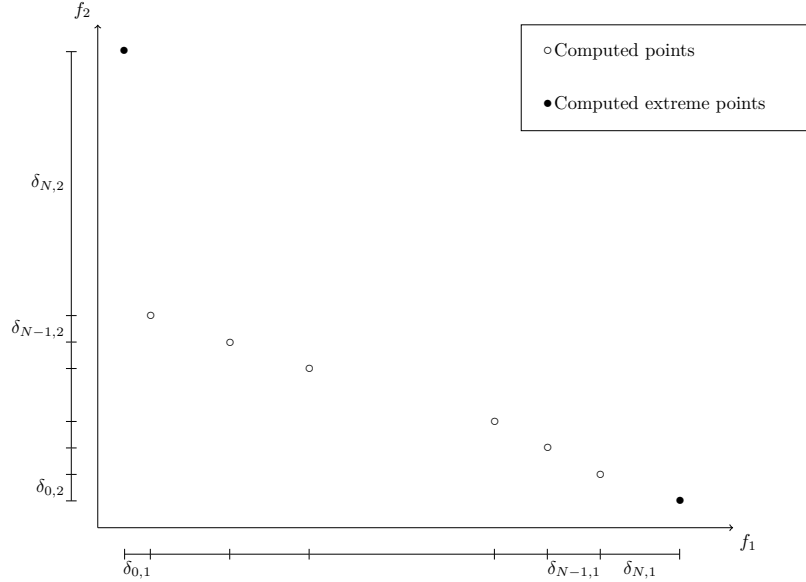
Figure 4: Illustration of the \Gamma metric for a biobjective problem (inspired by [34])
