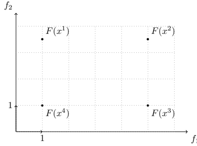
Figure 2: Example of the dominance relation for objective vectors for a biobjective problem (inspired by [10]): x^4 \prec\prec x^2 , x^4 \prec x^2 , x^4 \preceq x^2 , x^1 \prec x^2 , x^3 \prec x^2 , x^4 \preceq x^1 , x^4 \preceq x^3 , x^4 \preceq x^1 , x^1 \preceq x^1 , x^2 \preceq x^2 , x^3 \preceq x^3 , x^4 \preceq x^4 and x^1 \parallel x^3
