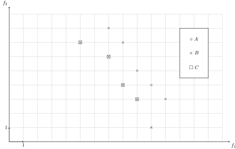
Figure 3: Example of the dominance relation for Pareto set approximations in the objective space for a biobjective problem (inspired by [10]): C \prec A , B \prec A , B \prec\prec A , B \prec C , B \preceq C , C \preceq A , B \preceq A , A \preceq A , B \preceq B , C \preceq C , C \triangleleft A , B \triangleleft A and B \triangleleft C
