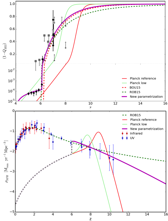
Fig. 2. Upper panel: reionisation histories compared to low-redshift probes. Same as Fig. 1 with the magenta curve displaying the best-fit from the parameterization. Lower panel: same as Fig. 1 with the magenta curve showing the associated derived \rho_{\text{SFR}} .
