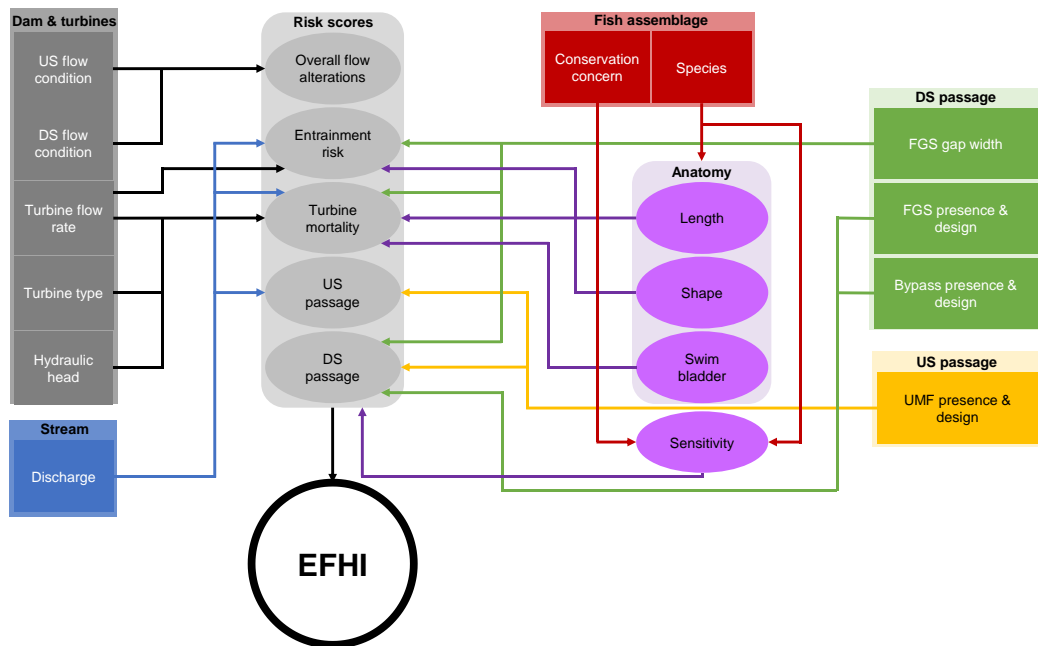
Fig. 15.1 Mechanistic model of the European Fish Hazard Index components. Rectangles = input parameters, ellipses = derived variables, open circle = final
