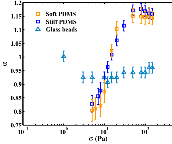
FIG. 9. \alpha parameter (Eq. (19)) versus shear stress.
