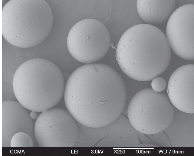
FIG. 4. Electron micrograph of manufactured stiff PDMS particles.
