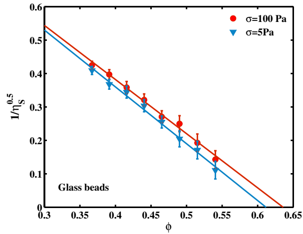
FIG. 8. Inverse of the square root of the reduced viscosity versus particle volume fraction for several shear stress values.
