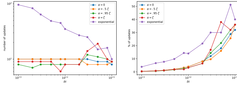
Figure 2: Polynomial matrix case: Number of updates with respect to the time-step, total value (left), percentage of the discretization times (right).
