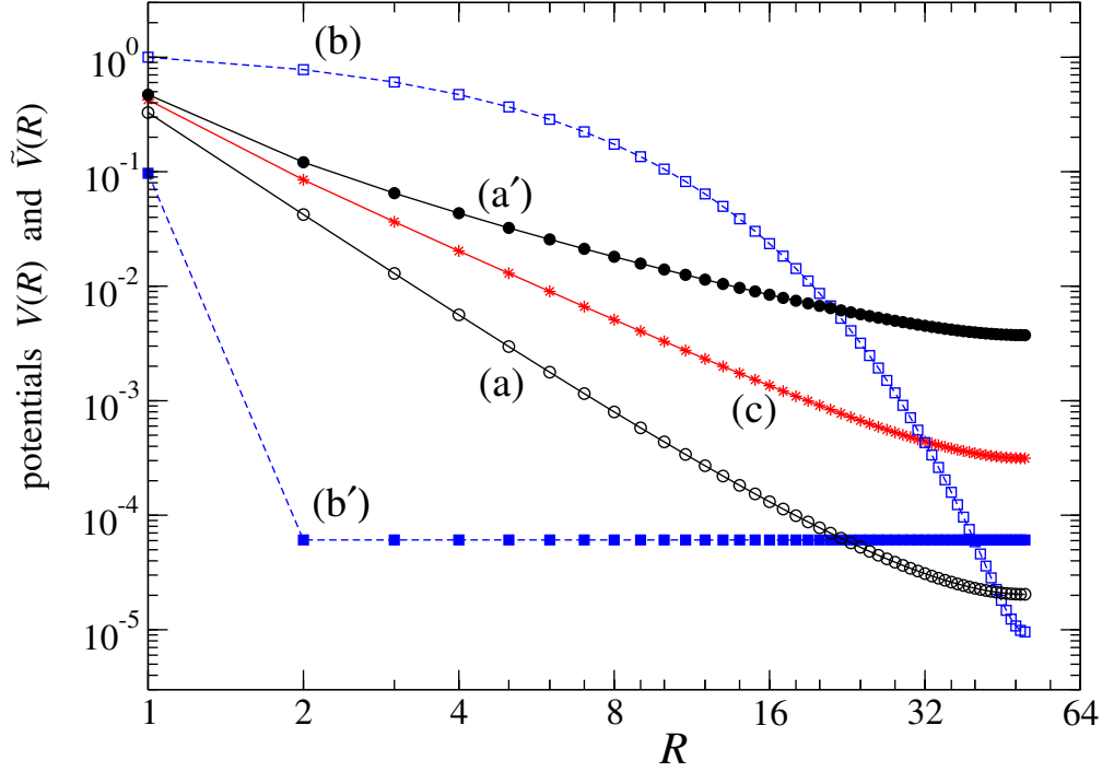
Figure 1: Three examples of a potential V(R) and its dual \tilde{V}(R) on a ring of N = 100 sites. (a) Open black circles: The power law potential V(R) = \pi^{-1}N^3/[R(N-R)]^3 , appropriately symmetrized to satisfy equation (6); for N \rightarrow \infty it tends to V(R) = 1/(\pi R^3) . (a'): Its dual (filled black circles); for N \rightarrow \infty it tends to a potential that decays with distance as \sim 1/R . (b) Open blue squares: The exponential potential V_{\text{exp}}(R) of equation (22) for \alpha = 0.25 . (b'): Its dual (filled blue squares), equations (23) and (24). (c) Red stars: The self-dual potential V(R) = \tilde{V}(R) = V^*(R) , equation (72).
