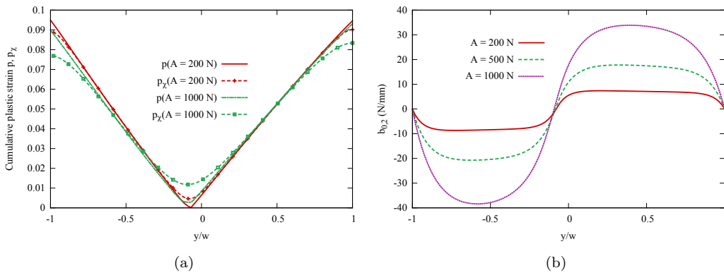
Fig. 10: (a) Cumulative plastic strain and associated micromorphic variable along the cross section at x = 0 ; (b) the generalized stress component b_{0,2} along the cross-section at x = 0 . Material parameters: R_0 = 100 MPa, H_\chi = 10^4 MPa, H = 0 . Applied curvature \kappa = 0.0348 mm ^{-1} .
