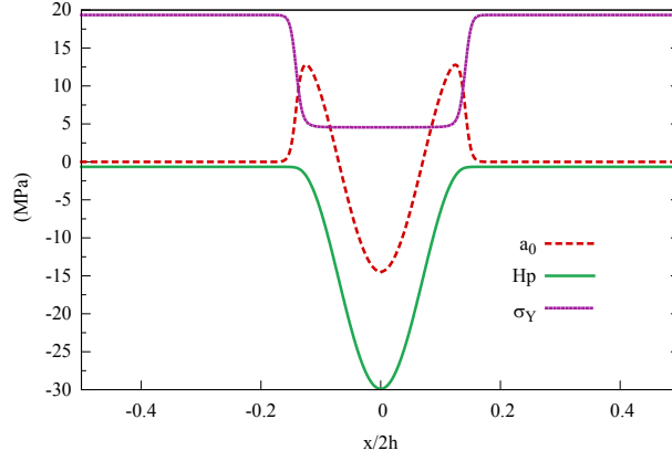
Fig. 16: Radius \sigma_Y of the yield surface, the generalized stress a_0 and the contribution of the linear softening term Hp along the strip length ( \bar{F}_{12} = 0.12 ); R_0 = 20 MPa, H = -20 MPa, H_\chi = 10^5 MPa, A = 4 N, h = 5 mm.
