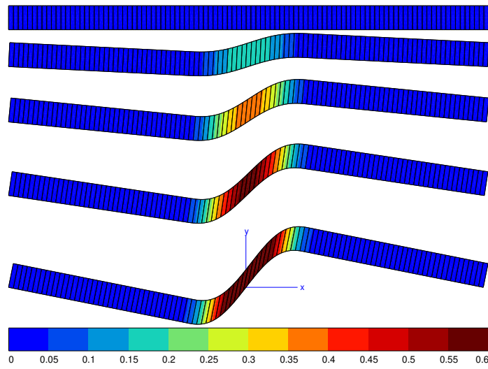
Fig. 28: Finite element simulation of shear localization in a micromorphic strip. Deformed states \bar{\gamma} = 0.; 0.05; 0.1; 0.15; 0.2 , from top to bottom, respectively. The fields of plastic microstrain p_\chi are also given. The parameters of the simulation are given in Table 5.
