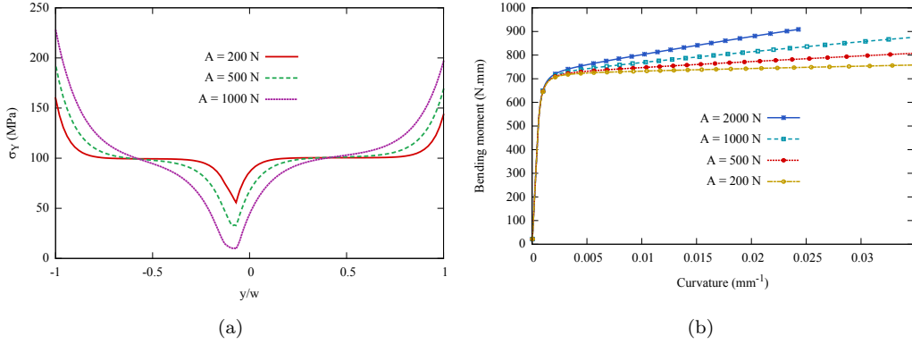
Fig. 11: (a) The radius of yield surface \sigma_Y = R_0 + H_\chi(p - p_\chi) captured at \kappa = 0.0348 \text{ mm}^{-1} ; (b) the bending moment-curvature curve. Material parameters: H_\chi = 10^4 \text{ MPa} , R_0 = 100 \text{ MPa} , H = 0 .
