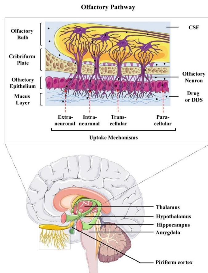
Figure 1. Uptake mechanisms involved in the transport of therapeutic proteins from the nasal cavity directly to the brain via the olfactory nerve pathway (Reprinted with permission from Ref [70]. Copyright 2018 Elsevier)
