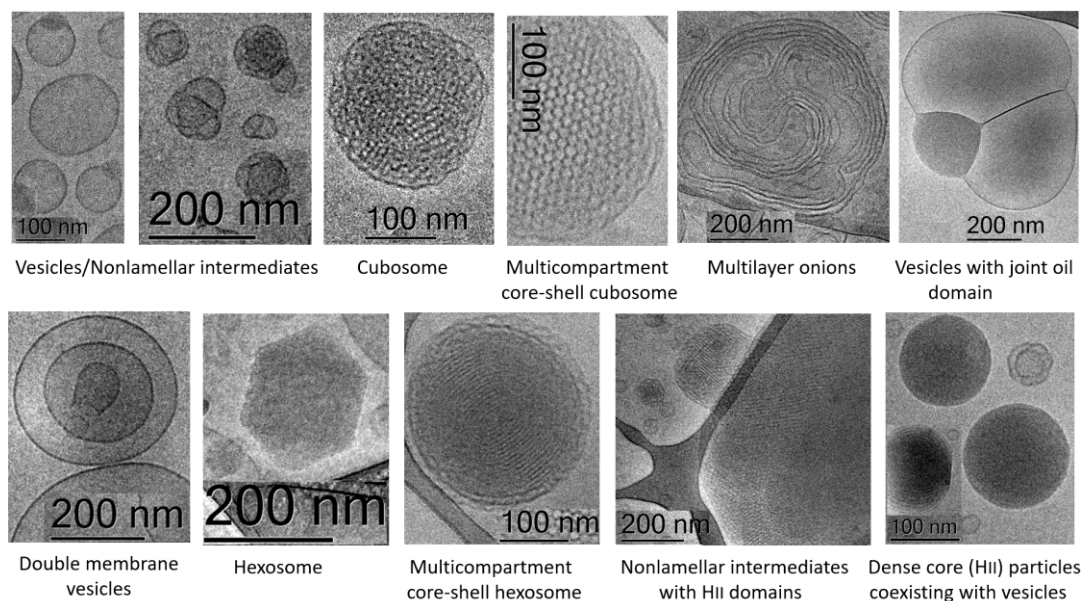
Figure 11. Cryo-TEM images of lipid nanoparticles obtained by self-assembly of custom-synthesized plasmenyl (ether) and ester phospholipids with long PUFA (22:5 n6) chains and the nonlamellar lipid monoolein. The liquid crystalline nanoparticle topologies and the compartmentalized biomimetic supramolecular architectures comprise vesicles, cubosomal intermediates, cubosomes coexisting with vesicles, multicompartment core-shell cubosomes and hexosomes, multilayer onions; vesicles with joint oil domains, double membrane vesicles, nonlamellar intermediates with H_{II} domains, and dense core ( H_{II} ) particles hexosomes coexisting with vesicles. (Reprinted from Ref [190]. Frontiers Open Access 2021)
