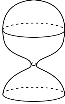
FIGURE 3. \tilde{\Sigma}^\varepsilon range by u^\varepsilon of a neighbourhood of the highest bubble
