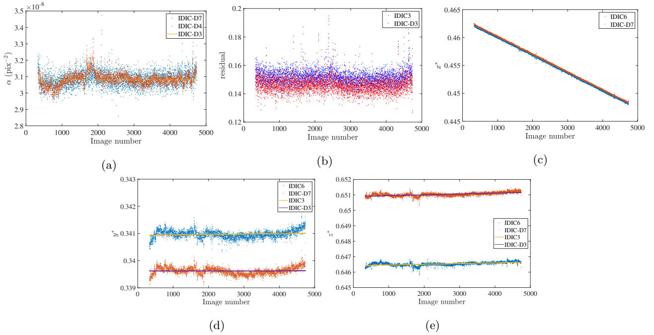
Figure 7: Calibration result profiles of IDIC and IDIC-D on the same EBSD line scan data. (a) Calibrated barrel parameter \alpha ; (b) Residuals of image correlations; Projection center coordinates x^* (c), y^* (d), z^* (e).
