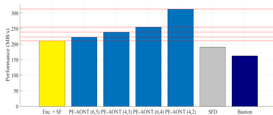
Figure 6: Performance benchmark. PE-AONT was measured in different configurations of (k, e) . In all of them it is faster than encryption and straightforward fragmentation (enc.+ SF). It is also faster than two fragmentation schemes protecting against data exposure: secure fragmentation and dispersal (SFD) and the Bastion scheme.
