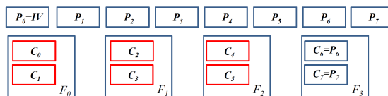
Figure 2: Step 1 example with k = 4 , e = 3 , and l = 8 . The first step of the algorithm fragments D into k fragments of f = 2 blocks, the last fragment contains plaintext blocks. D has 7 blocks: D = P_1, P_2, \dots, P_7 . The block P_0 = IV is added to D ; it corresponds to the ciphertext block containing the Initial Vector used by the cipher.
