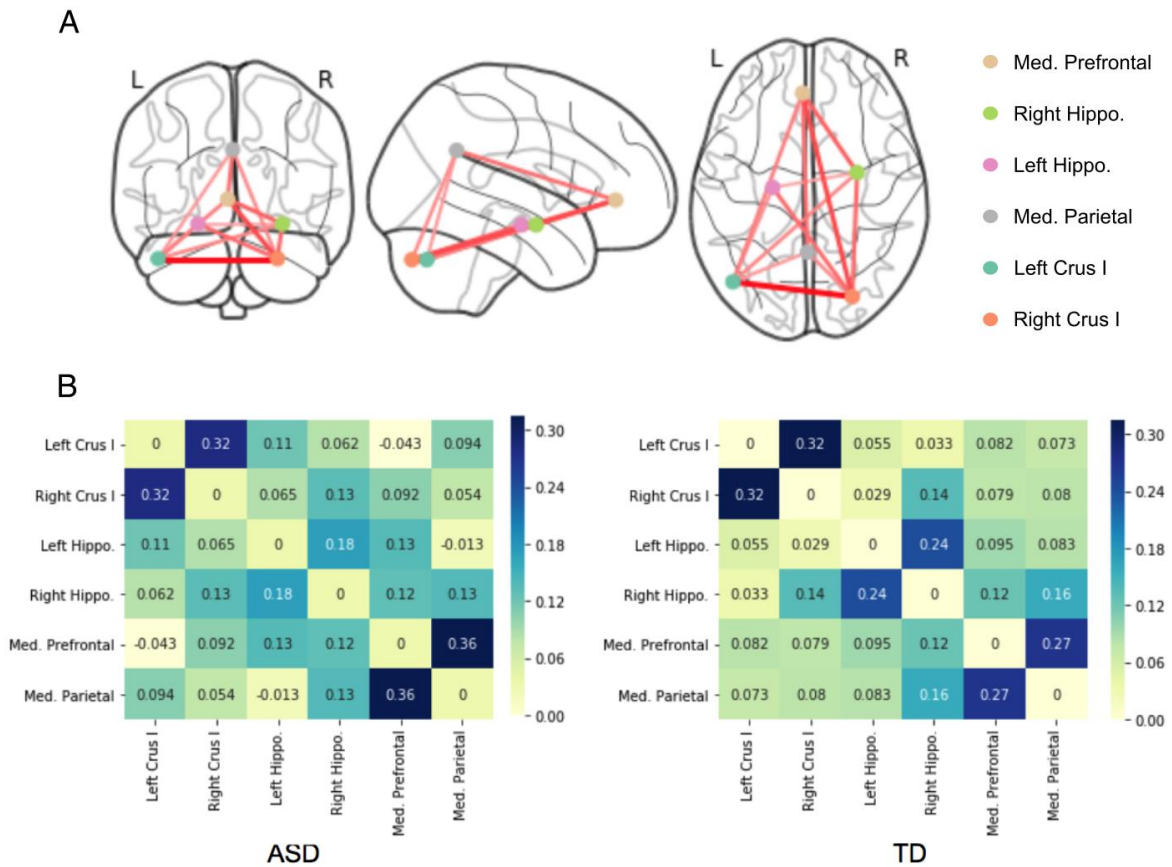
Figure 4: Cerebellum, hippocampus, medial parietal, and medial prefrontal functional connectivity. (A) Representation of cerebellar functional connectivity between cerebellum, hippocampus, medial prefrontal and medial parietal cortex on a glass brain. Left Crus I (dark green), Right Crus I (orange), Left hippocampus (purple), Right Hippocampus (light green), Medial parietal cortex (gray), Medial prefrontal cortex (golden); the thickness and color intensity of the in-between segments represent the correlation strength. (B) Correlation matrices between the regions of interest (see A) in the ASD and TD group. Hippo: hippocampus; Med. Prefrontal: medial prefrontal cortex; Med. Parietal: medial parietal cortex. ASD: Individuals with autism spectrum disorder; TD: Individual with typical development.
