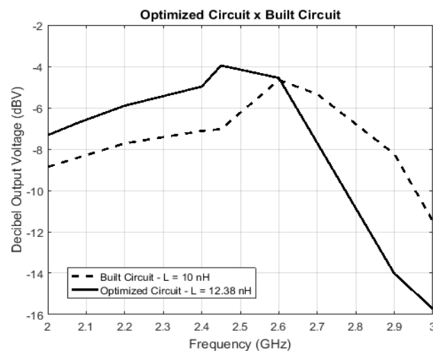
Fig. 17. Simulation of the Optimization Circuit ( L = 12.38 \text{ nH} ) and Simulation of Built Circuit ( L = 10 \text{ nH} ).
