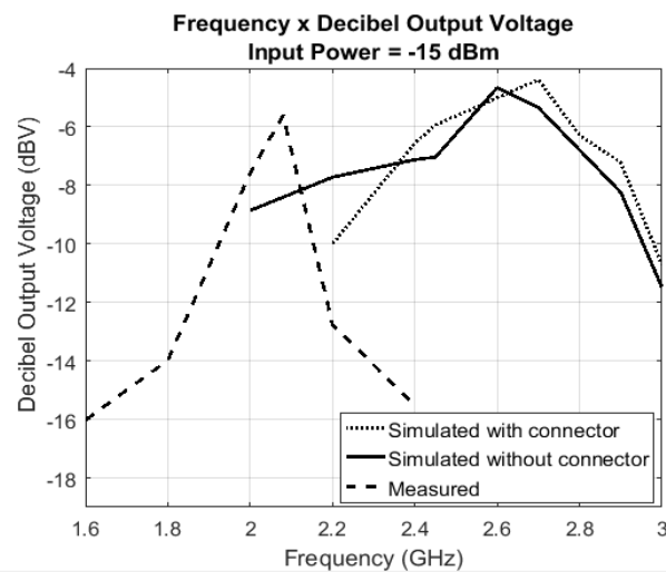
Fig. 16. Frequency x Decibel Output Voltage: Measurements and Simulations - P_{in} = -15 \text{ dBm} .
