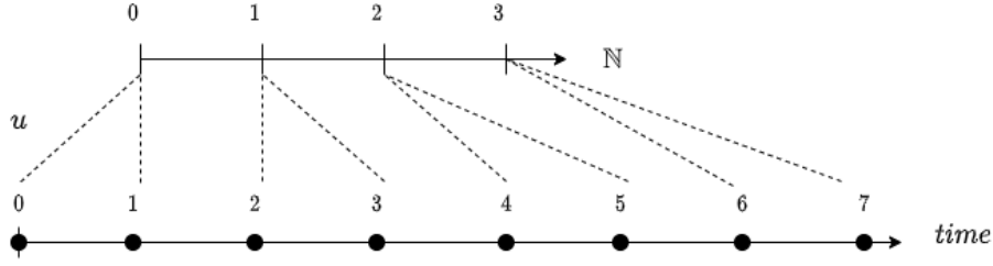
Figure 1: Time modelling.
