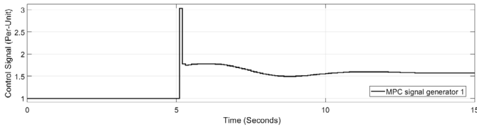
Fig. 6. MPC signal applied to generator one after t = 5s
