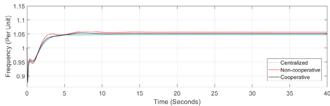
Fig. 14. Frequency response for the first generator using the three control approaches
