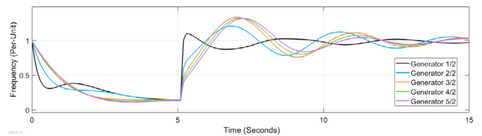
Fig. 11. Per-unit frequency before and after active the predictive control signal at t = 5s with a cooperative distributed approach.
