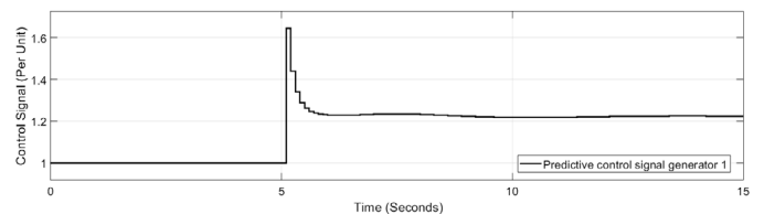
Fig. 12. MPC signal applied to generator one after t = 5s
