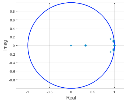
Fig. 4. Eigenvalues of Koopman Matrix for generator one
