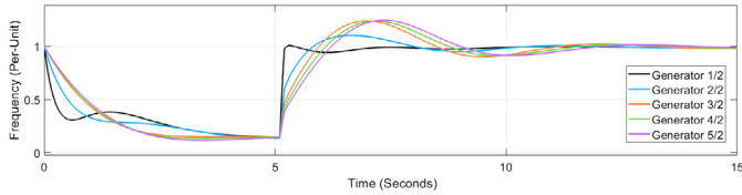
Fig. 5. Per-unit frequency before and after active the predictive control signal at t = 5s with decentralized approach.
