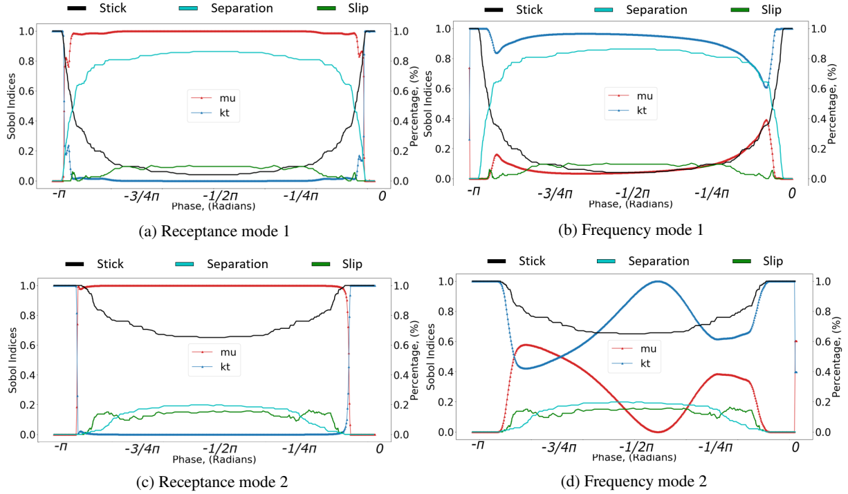
Figure 7: Sobol indices for accelerance, frequency with contact conditions superimposed
