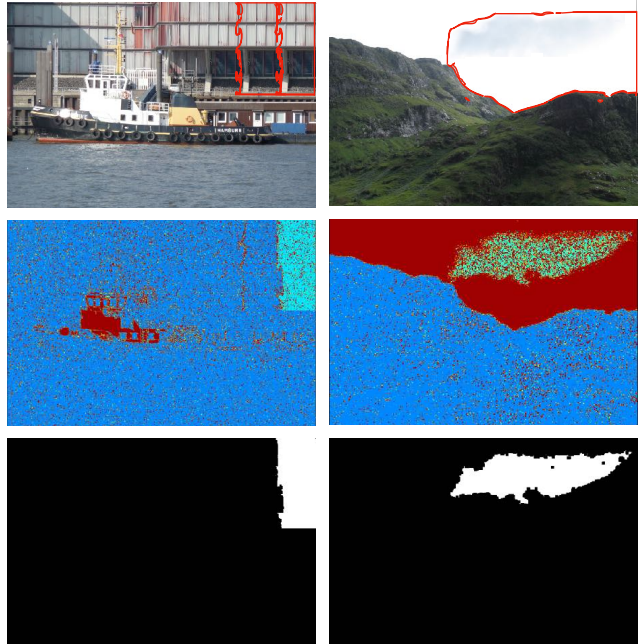
Figure 6: Up: images with tampered regions indicated in red. Middle: grid origin vote maps. Down: detected forgery masks. On the left, an example of a missed detection: one of the two forged regions was not detected because its local grid was correctly aligned with the global grid. On the right, an incomplete detection caused by saturation in the image.
