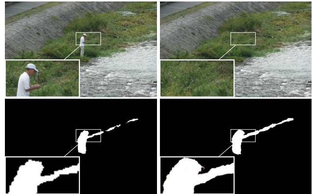
Figure 1: Result of the proposed method, from top left to bottom right: original image, forged image (input of the method), detected forgeries, ground-truth. The fisherman and the fishing rod have been removed. The resulting detected mask does not require visual interpretation.
