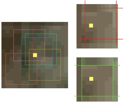
Figure 2: Each pixel (yellow) belongs to 64 different 8 \times 8 blocks of the image. Six of them were drawn in different colors on the left. Top right shows (in red) the position of a patch not aligned with the grid. Bottom right shows (in green) the position of the patch containing the pixel matching the JPEG grid.
