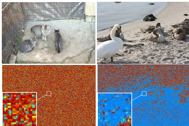
Figure 3: Left: Uncompressed image and its vote map. Right: JPEG compressed image and its vote map. In both cases, the pixels which return a NON VALID vote (a tie) are shown in dark red.
