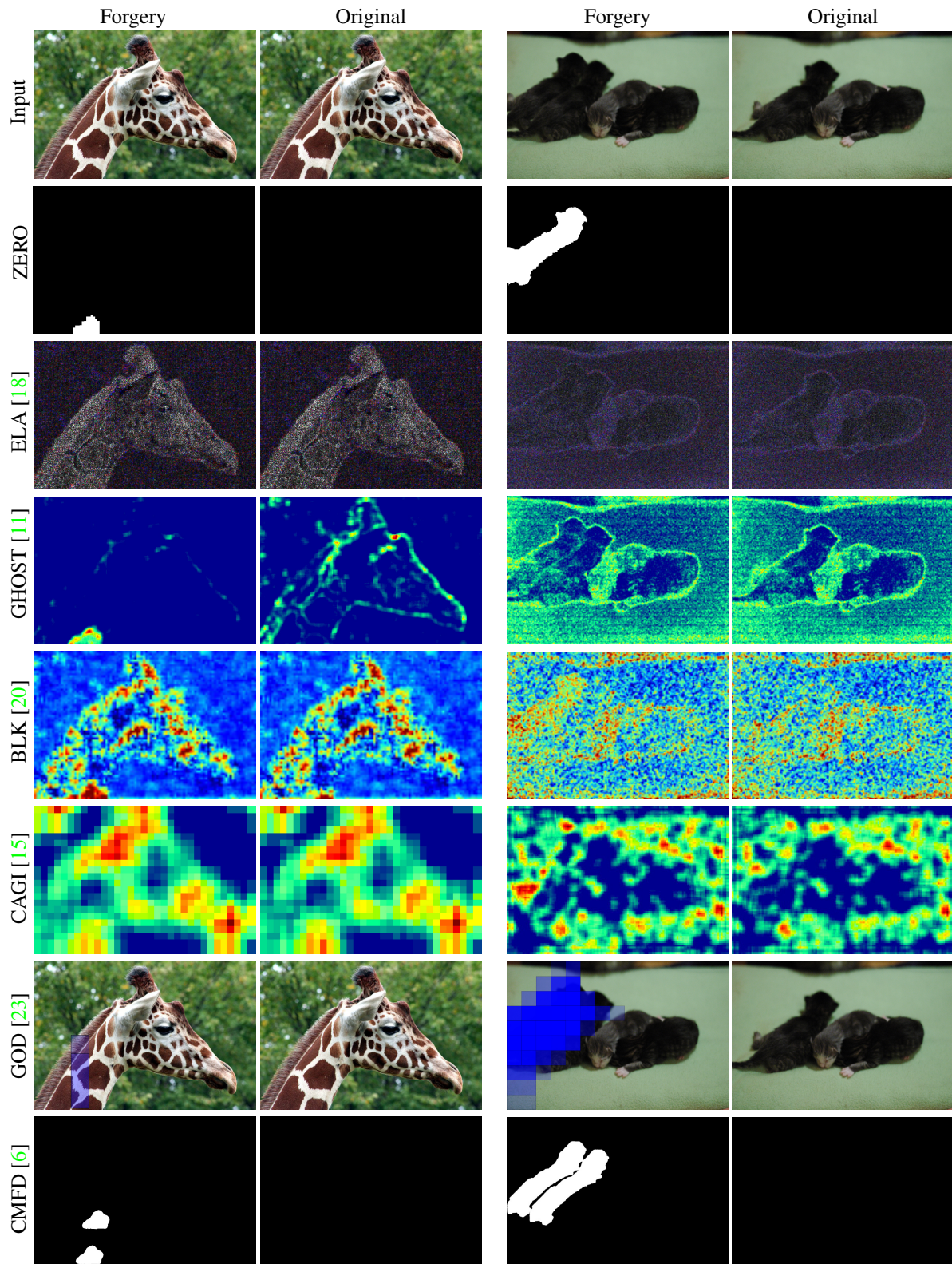
Figure 7: Results of the proposed method compared to the JPEG state-of-the-art methods. The first one produces a difference image, the three following heat maps and the last two masks. The methods are applied to the forged image and also its original source.
