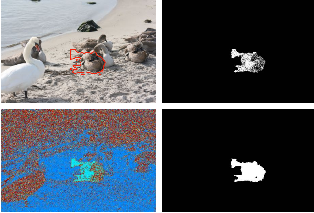
Figure 5: Up-left: an image with a tampered region indicated in red. Down-left: grid origin vote map. Up-right: raw forgery mask. Down-right: final forgery mask after holes filled by a mathematical morphology closing operation.
