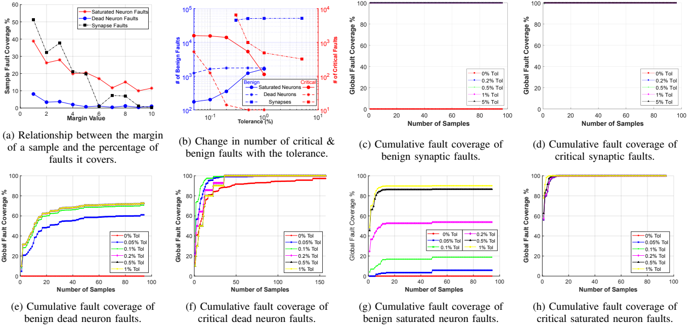
Fig. 9: N-MNIST SNN.
