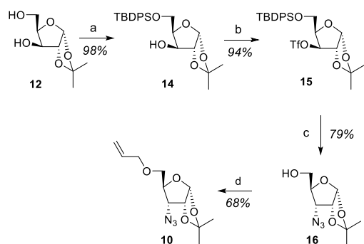
Scheme 2. Reagents and conditions: (a) TBDPSCI, imidazole, DMAP, DCM, r.t., 2 h; (b) Tf 2 O, pyr., DMAP, DCM, r.t., 2 h; (c-i) NaN 3 , n Bu 4 NBr, DMF, M.W. 80 °C (25 W), 10 min; -ii) TBAF, THF, r.t., 30 min; (d) NaH, allyl bromide, THF, r.t., 2 h.
