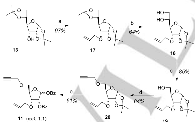
Scheme 3. Reagents and conditions: (a) NaH, allyl bromide, THF, r.t., 3 h; (b) Acetic ac./formic ac./H 2 O, r.t.; (c-i) NaIO 4 , EtOH/H 2 O, r.t., 1 h; -ii) NaBH 4 , EtOH, r.t., 30 min; (d) NaH, propargyl bromide, THF, r.t., 3 h; (e-i) Formic ac./H 2 O, 60 °C, 1 h; -ii) BzCl, Pyr., DMAP, DCM, r.t., 2 h.
