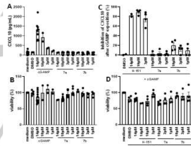
Figure 2. Biological evaluation of compound 7a and 7b tested as STING agonist (A, B) or antagonist (C, D) on bone marrow derived macrophages. Reference agonist cGAMP and antagonist H151 are shown. In C, D the compounds are added 3hr prior to macrophage stimulation with cGAMP (14 \mu M). Compounds cytotoxicity is evaluated by MTT assay. Data are from 4 (A, B) or 3 (C, D) independent experiments, each point representing an independent bone marrow culture from an individual mouse.
